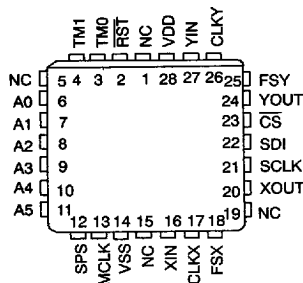
28-Pin PLCC
