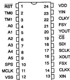
24-Pin DIP (600 MIL)
