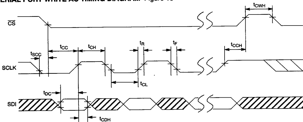
SERIAL PORT WRITE AC TIMING DIAGRAM Figure 13
