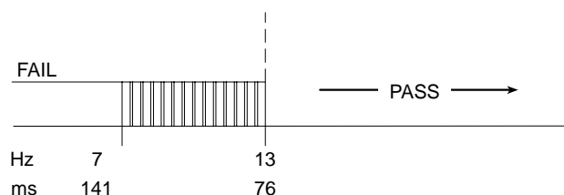
Figure 20. WDI Signal for C_{Delay} = 0.82 \mu\text{F} using CS8141
