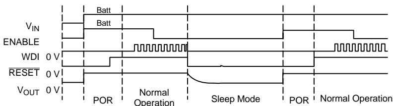
Figure 16. Timing Diagrams for Watchdog and ENABLE Functions
