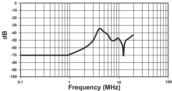
Transhybrid Loss
