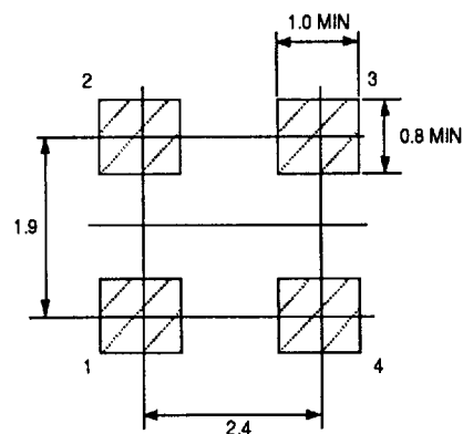
PACKAGE OUTLINE 39 RECOMMENDED P.C.B. LAYOUT
