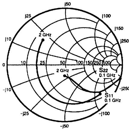
Coordinates in Ohms Frequency in GHz ( V_{CE} = 10\text{ V} , I_C = 5\text{ mA} )
