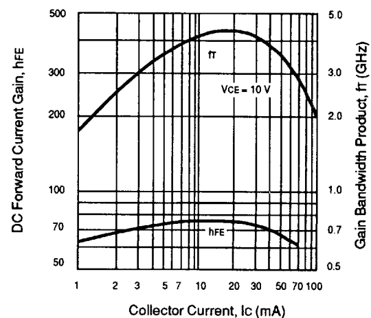
GAIN BANDWIDTH PRODUCT AND FORWARD CURRENT GAIN vs. COLLECTOR CURRENT
