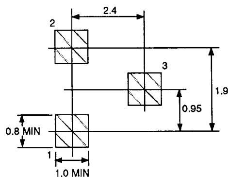
PACKAGE OUTLINE 33 RECOMMENDED P.C.B. LAYOUT
