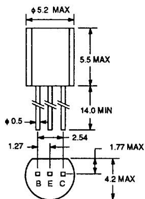
PACKAGE OUTLINE 32
