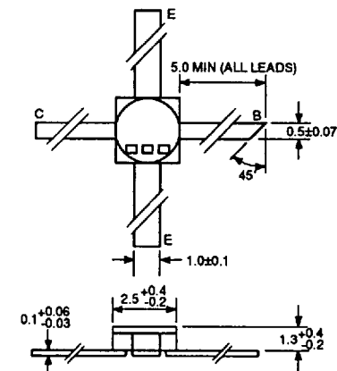
PACKAGE OUTLINE 07
