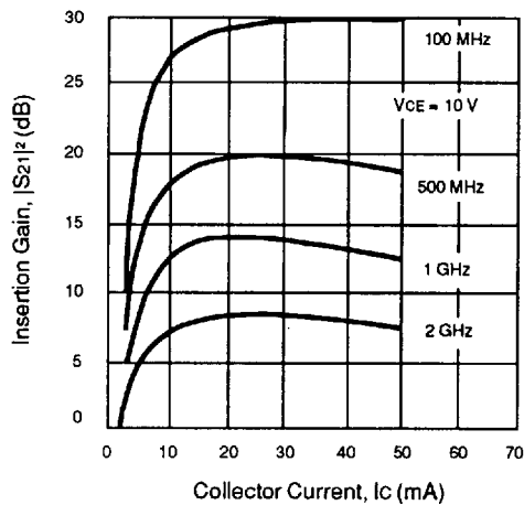
NE02107 INSERTION GAIN vs. COLLECTOR CURRENT
