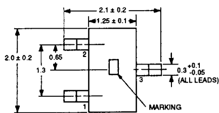
PACKAGE OUTLINE 30
