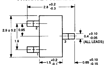
PACKAGE OUTLINE 33
