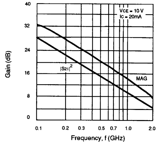
NE02133 GAIN vs. FREQUENCY
