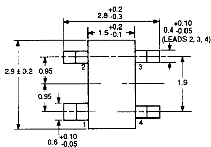
PACKAGE OUTLINE 39 (SOT-23)
