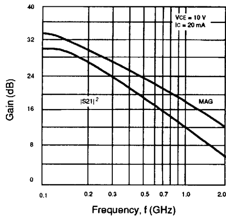
NE02107, NE02135 GAIN vs. FREQUENCY
