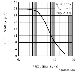
Power Bandwidth
