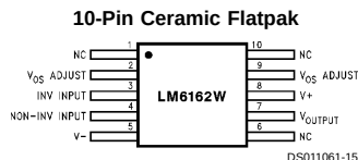
Top View See NS Package Number W10A
