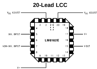
Top View See NS Package Number E20A
