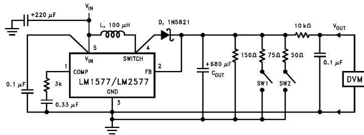
FIGURE 1. Circuit Used to Specify System Parameters for 12V Versions
