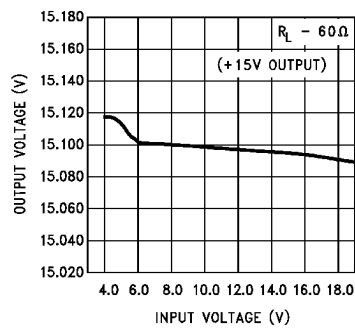
FIGURE 23. Line Regulation (Typical) of Flyback Regulator of Figure 22, +15V Output
