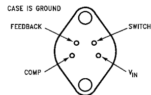
4-Lead TO-3 (K)
