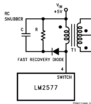
FIGURE 21. Snubber Circuit
