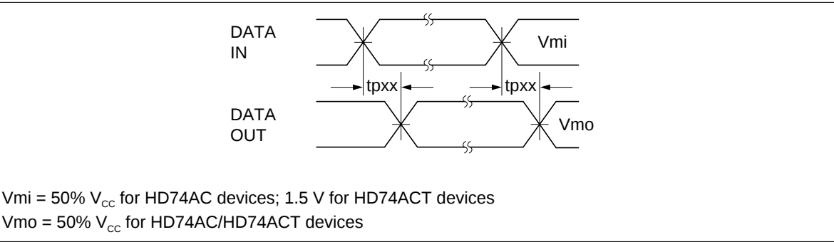
Figure 3 Waveform for Inverting and Non-Inverting Functions
