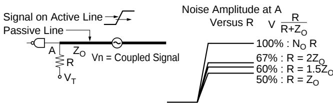
Figure 15 Effects of Termination on Crosstalk
