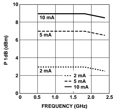
Figure 5. AT-31011 and AT-31033 Power at 1 dB Gain Compression vs. Frequency and Current at V_{CE} = 2.7V .
