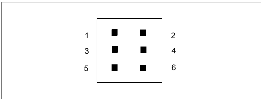
Figure 1-1. Jumper JP20
