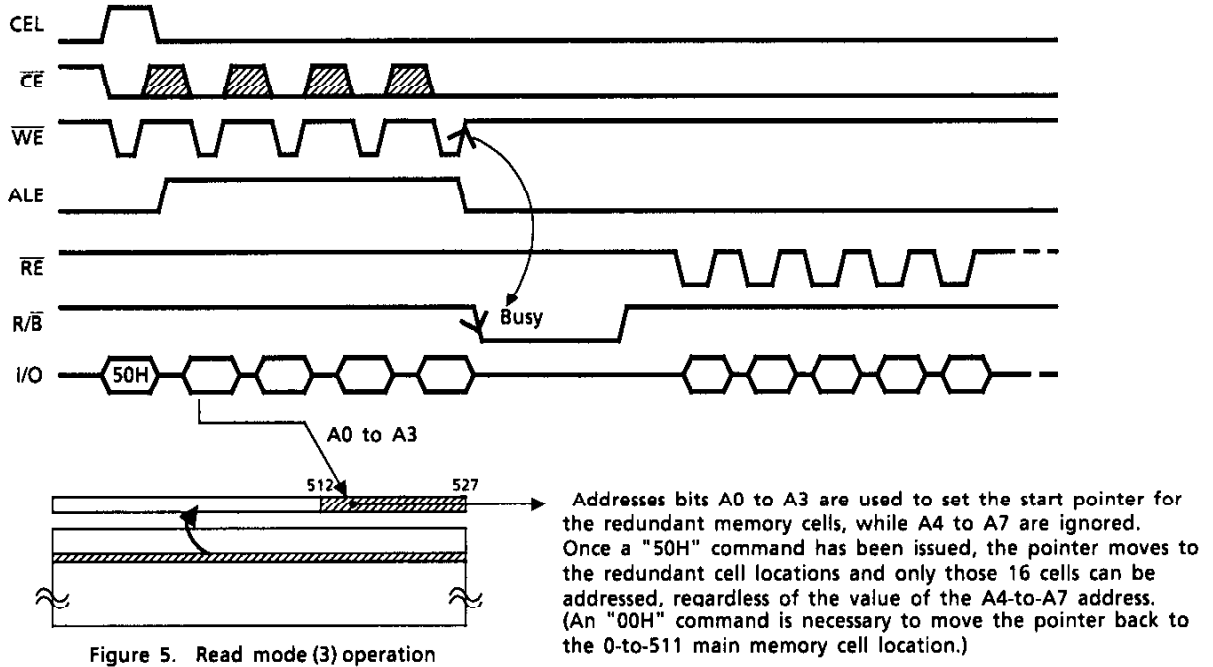
Figure 5. Read mode (3) operation
