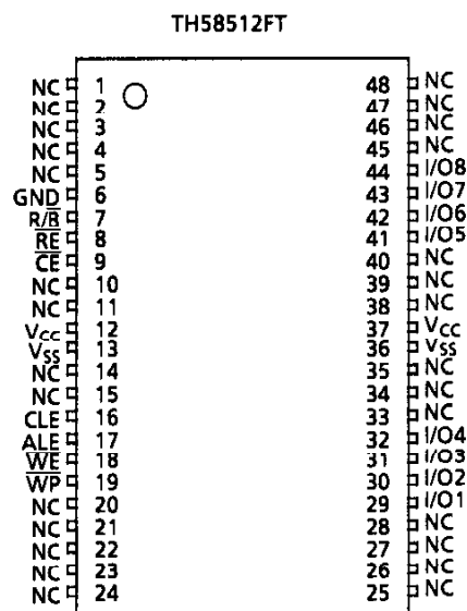
Figure 1. Pinout
