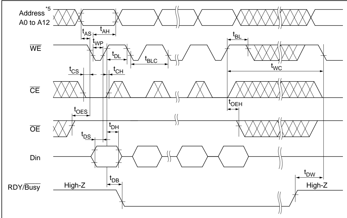
Page Write Timing Waveform(1) ( \overline{\text{WE}} Controlled)
