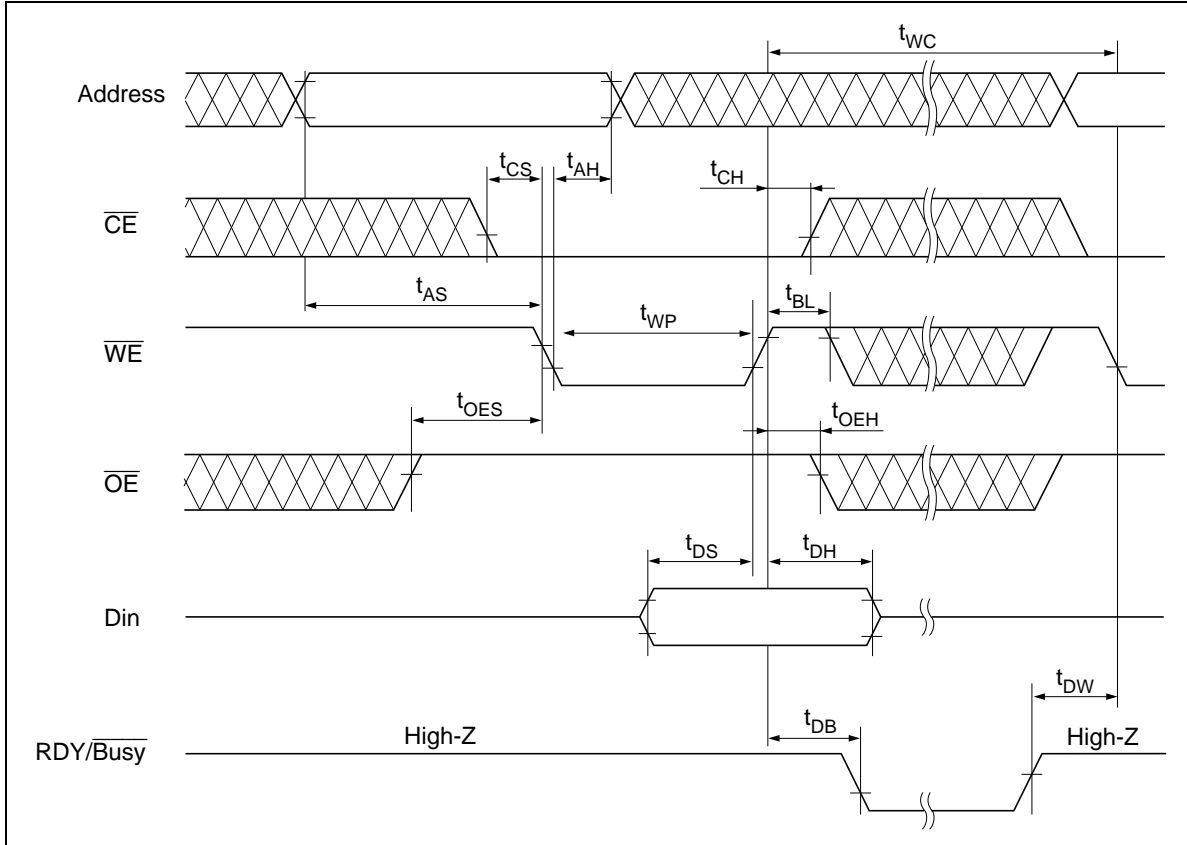
Byte Write Timing Waveform(1) ( \overline{\text{WE}} Controlled)
