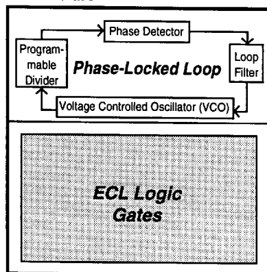
Figure 10. Q20000 "TURBO" + PLL Architecture
