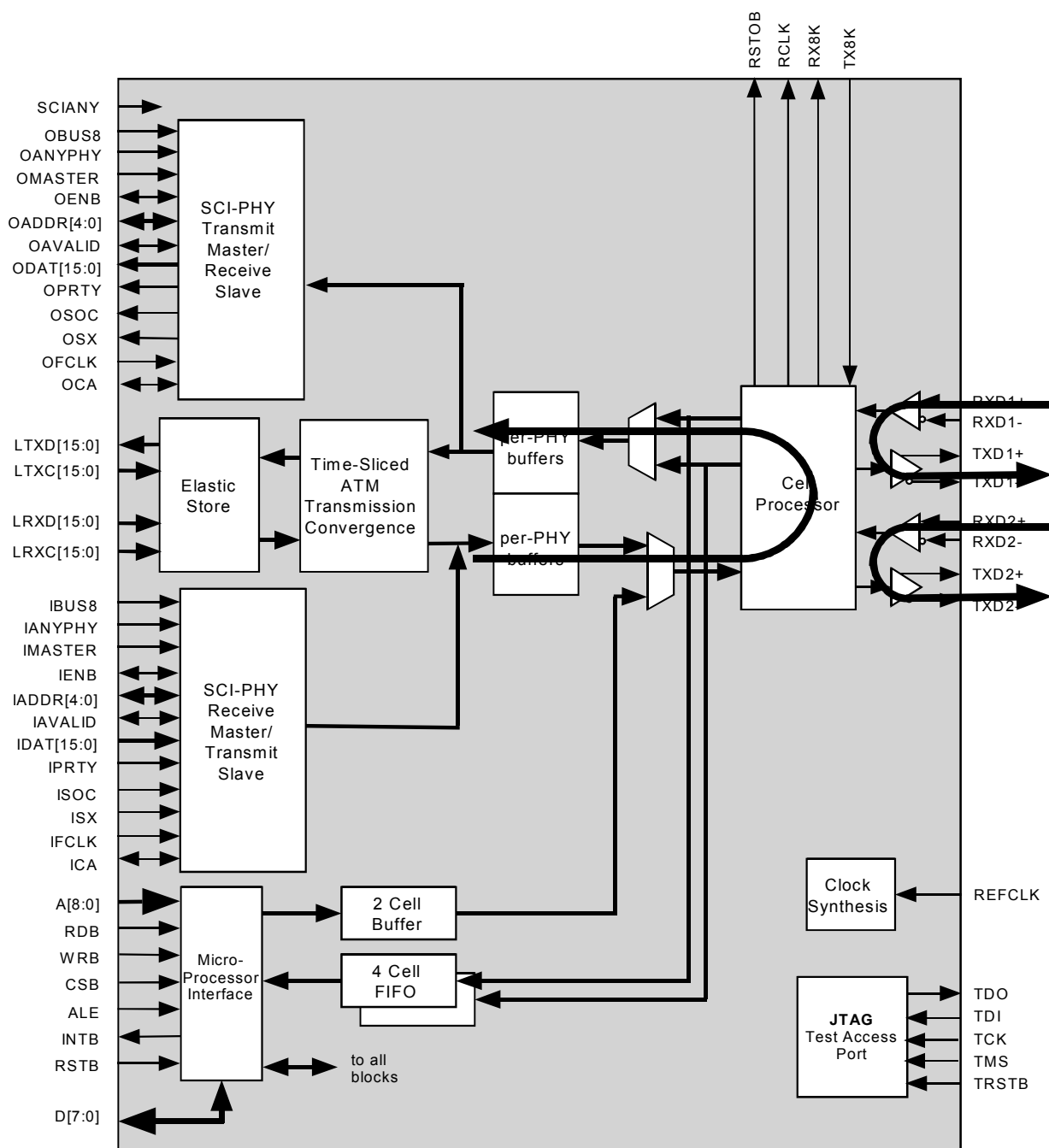
Fig. 10 Datapath Loopback
