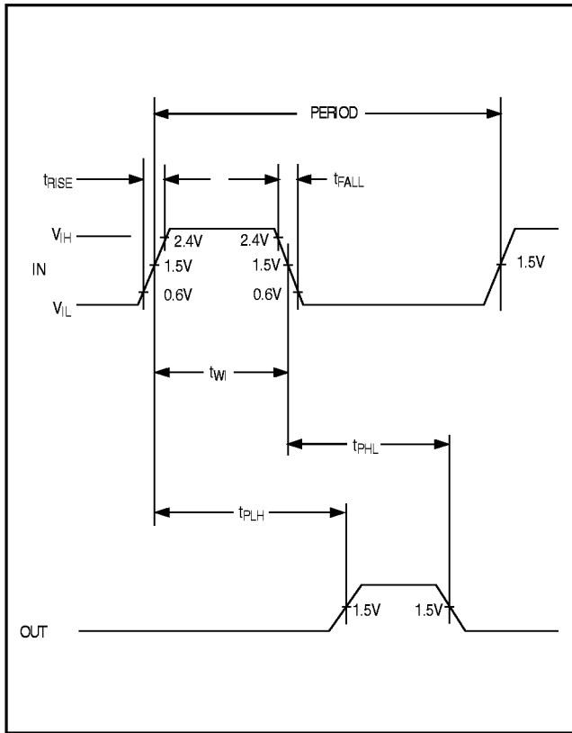
Figure 1. Timing Diagram
