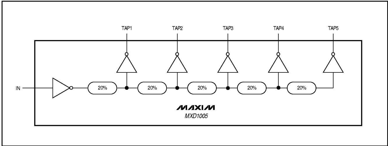
Functional Diagram
