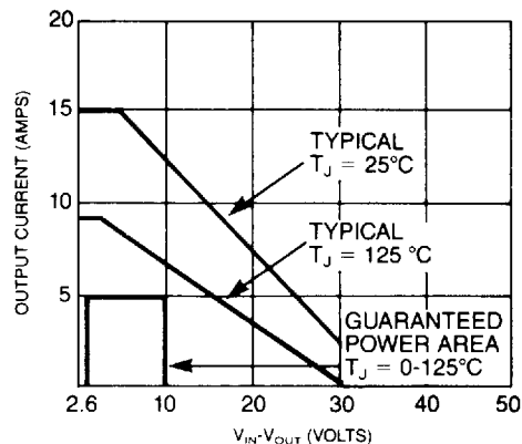
CURRENT LIMIT
