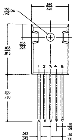
DEVICE OUTLINE F
