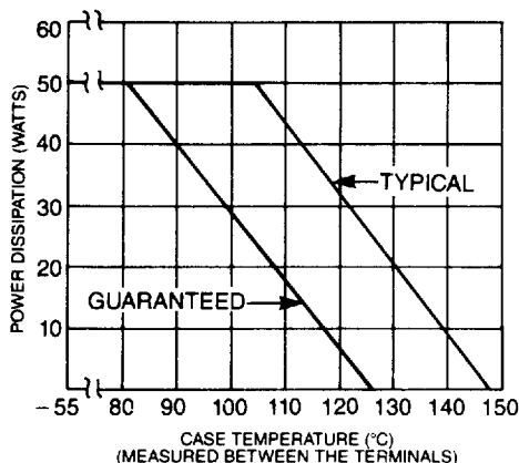
POWER DERATING
