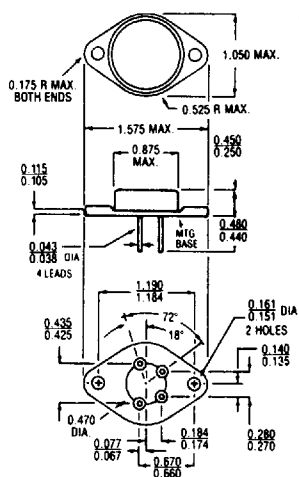
TO-3 (COPPER)
