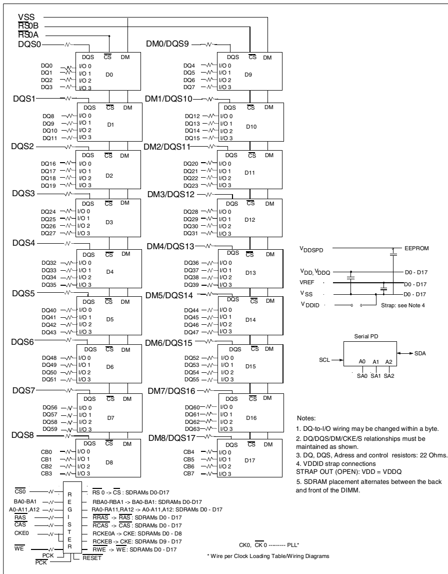
Block Diagram: One Bank 64M x 72 DDR-I SDRAM DIMM Modules (x4 comp.) HYS72D64500GR on Raw Card M
