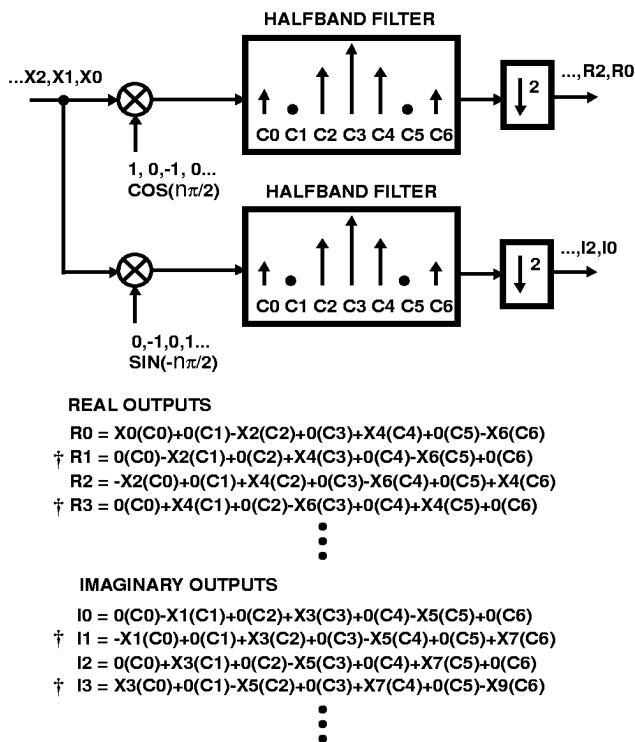
FIGURE 13. DOWN CONVERT AND DECIAMATE FUNCTION USING TRANSVERSAL FILTERS
