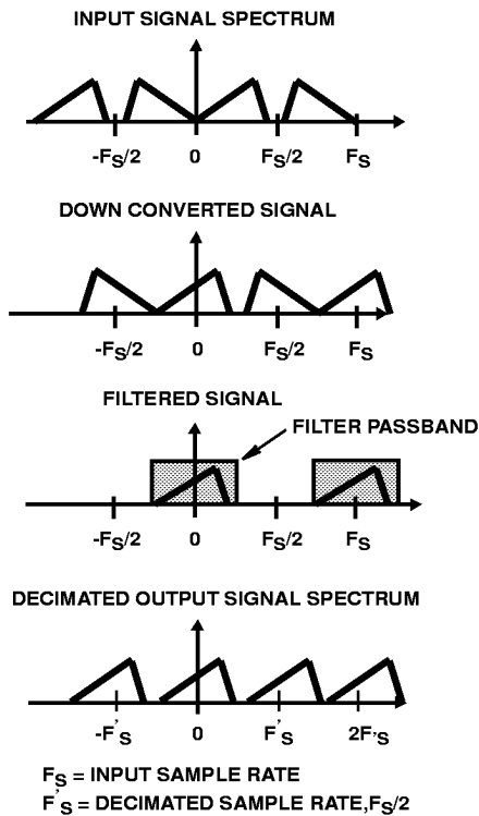
FIGURE 12. DOWN CONVERT AND DECIAMATE OPERATION
