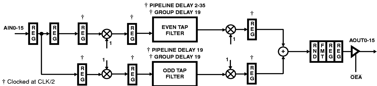
FIGURE 7A. DATA FLOW DIAGRAM FOR DECIMATE BY 2 FILTER MODE (INT/EXT = 1)
