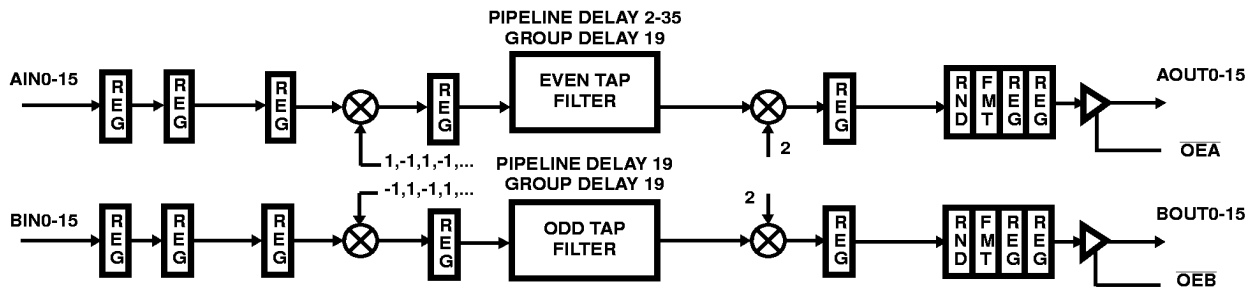
FIGURE 15B. DATA FLOW DIAGRAM FOR DOWN CONVERT AND DECIMATE MODE ( \text{INT/EXT} = 0 )
