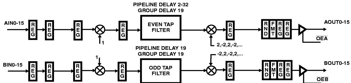
FIGURE 21B. DATA FLOW DIAGRAM FOR QUADRATURE TO REAL CONVERSION MODE ( \overline{\text{INT/EXT}} = 0 )
