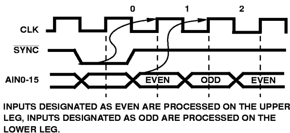
FIGURE 8. DATA SYNCHRONIZATION WITH PROCESSING LEGS ( \overline{\text{INT/EXT}} = 1 )
