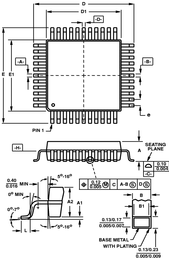
Q100.14x20 (JEDEC MO-108CC-1 ISSUE A) 100 LEAD METRIC PLASTIC QUAD FLATPACK PACKAGE
