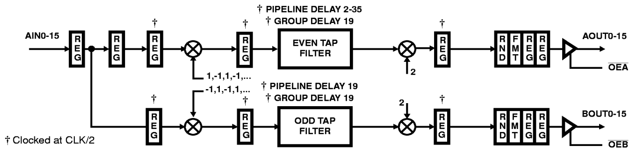
FIGURE 15A. DATA FLOW DIAGRAM FOR DOWN CONVERT AND DECIMATE MODE ( \text{INT/EXT} = 1 )
