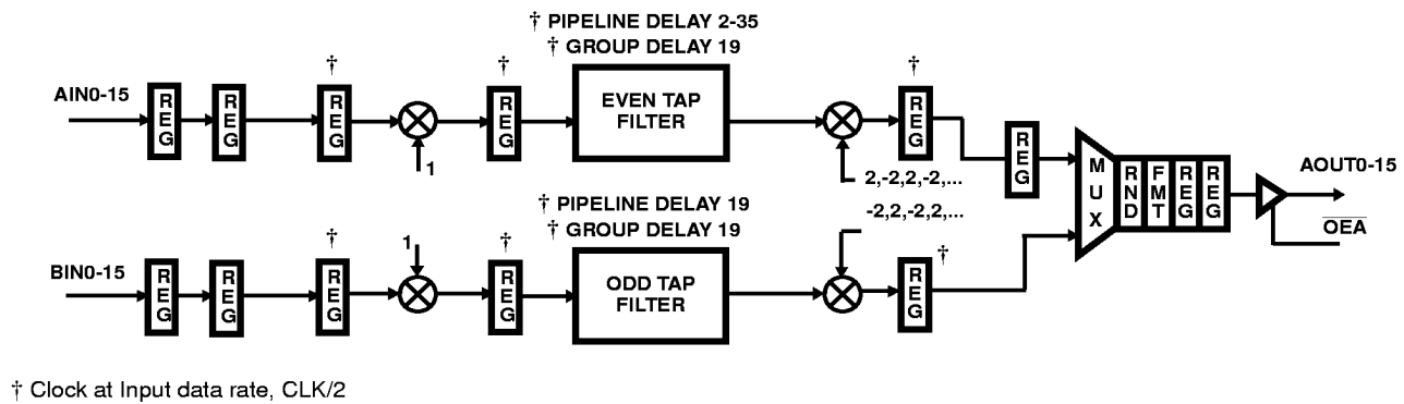
FIGURE 21A. DATA FLOW DIAGRAM FOR QUADRATURE TO REAL CONVERSION MODE ( \overline{\text{INT/EXT}} = 1 )
