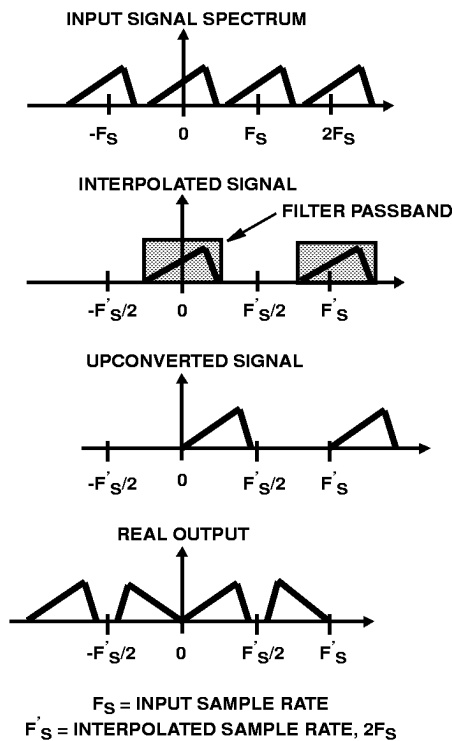
FIGURE 18. QUADRATURE TO REAL CONVERSION
