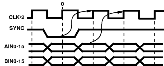
FIGURE 22. DATA SYNCHRONIZATION WITH PROCESSING LEGS ( \overline{\text{INT/EXT}} = 1 )
