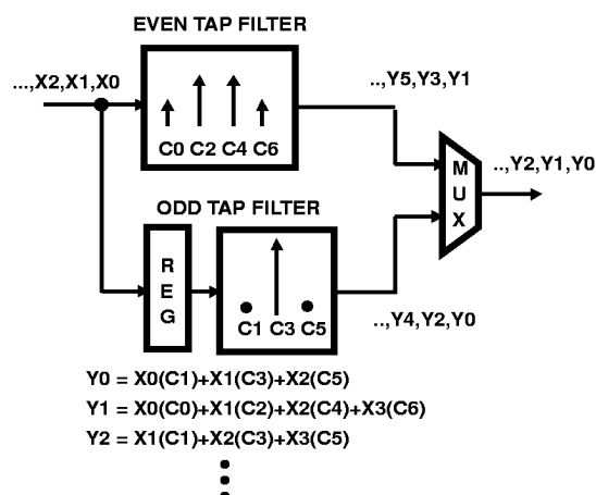
FIGURE 10. POLYPHASE IMPLEMENTATION OF INTERPOLATE BY TWO HALFBAND FILTER
