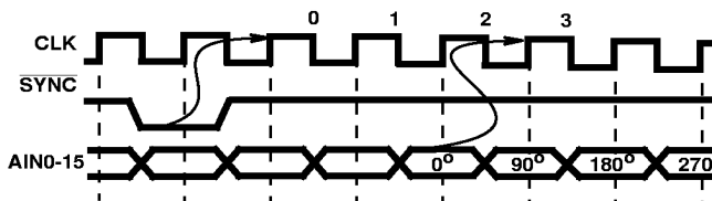
FIGURE 15B. DATA FLOW DIAGRAM FOR DOWN CONVERT AND DECIMATE MODE ( \text{INT/EXT} = 0 )
