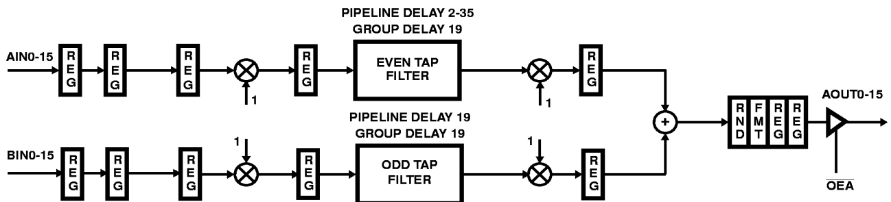
FIGURE 7B. DATA FLOW DIAGRAM FOR DECIMATE BY 2 FILTER MODE (INT/EXT = 0)
