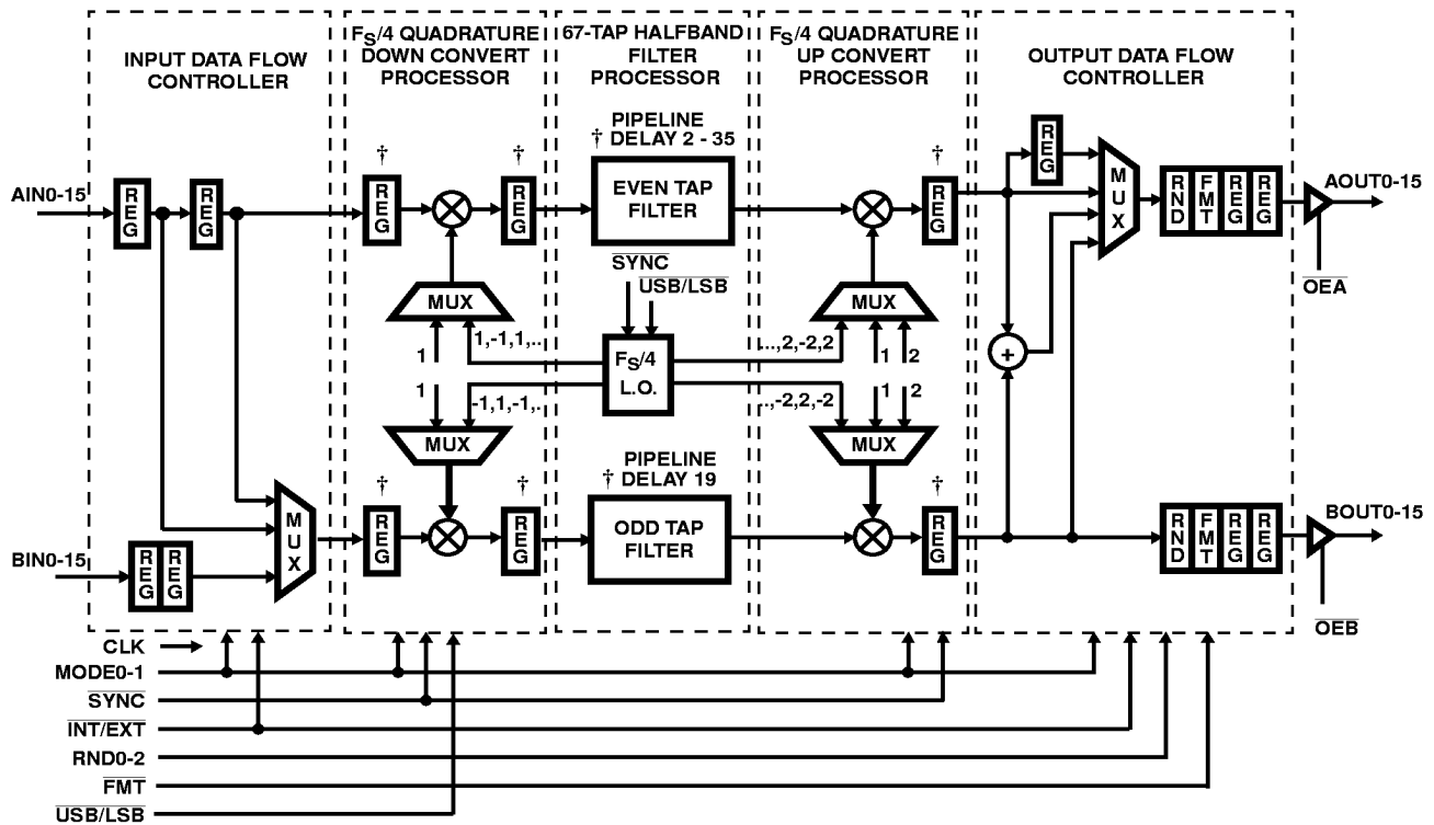
FIGURE 1. HALFBAND BLOCK DIAGRAM
