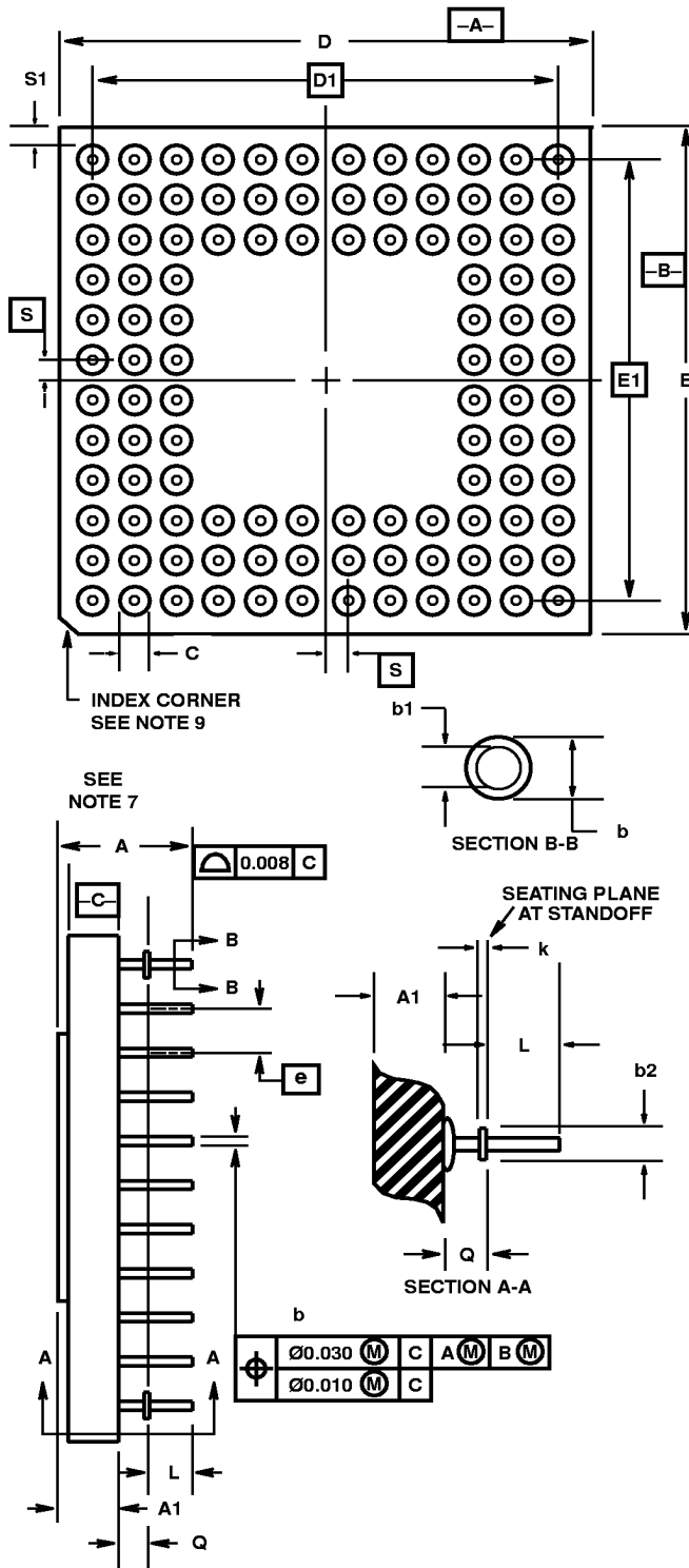
G85.A MIL-STD-1835 CMGA3-P85C (P-AC) 85 LEAD CERAMIC PIN GRID ARRAY PACKAGE
