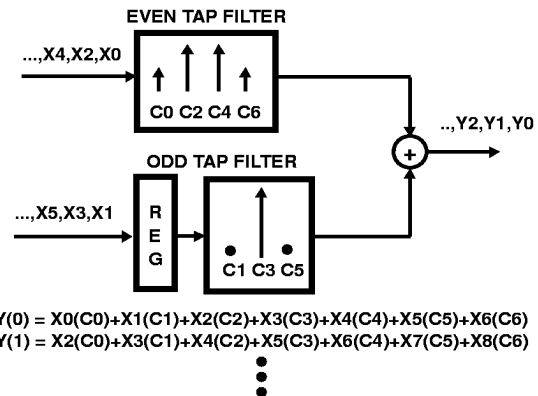
FIGURE 6. POLYPHASE IMPLEMENTATION OF DECIMATE BY 2 HALFBAND FILTER
