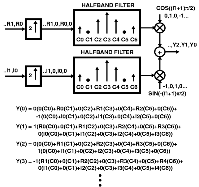
FIGURE 19. QUADRATURE TO REAL CONVERTER USING TRANSVERSAL FILTERS
