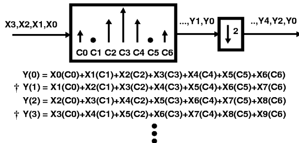
FIGURE 5. TRANSVERSAL IMPLEMENTATION OF DECIMATE BY 2 HALFBAND FILTER
