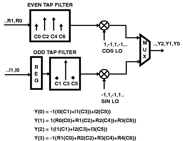
FIGURE 20. POLYPHASE IMPLEMENTATION OF QUADRATURE TO REAL CONVERTER
