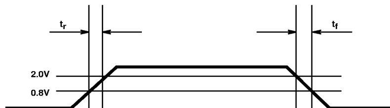
FIGURE 24. OUTPUT RISE AND FALL TIMES
