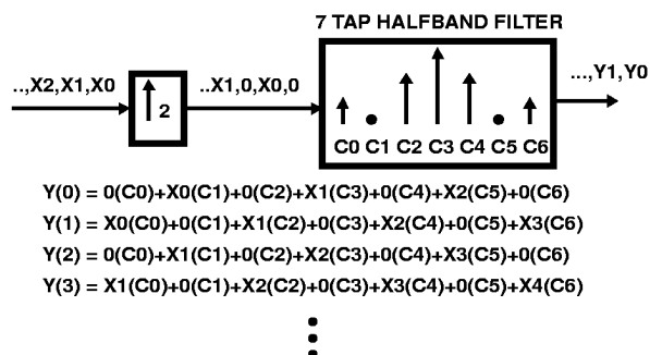
FIGURE 9. TRANSVERSAL IMPLEMENTATION OF INTERPOLATE BY TWO HALFBAND FILTER
