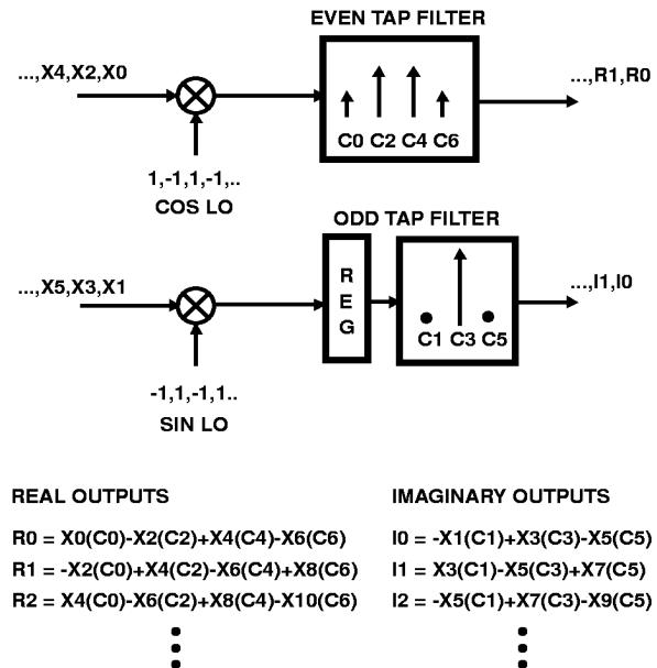
FIGURE 14. DOWN CONVERT AND DECIAMATE FUNCTION USING POLYPHASE FILTERS
