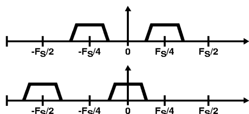
FIGURE 4. F_S/4 NEGATIVE SHIFT: DOWN CONVERSION
