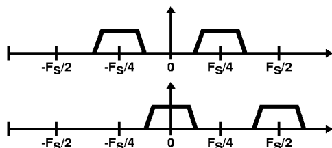
FIGURE 3. F_S/4 POSITIVE SHIFT: UP CONVERSION
