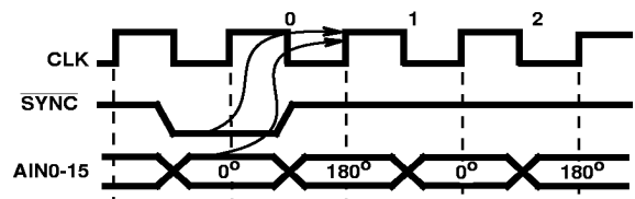
FIGURE 15B. DATA FLOW DIAGRAM FOR DOWN CONVERT AND DECIMATE MODE ( \text{INT/EXT} = 0 )
