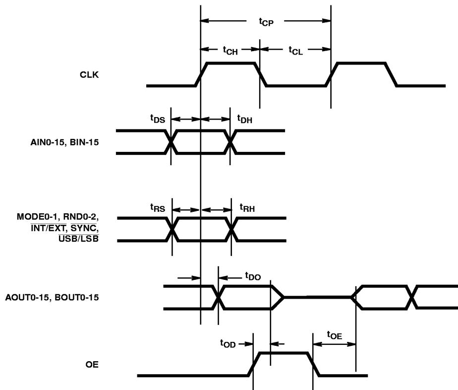
FIGURE 23. TIMING RELATIVE TO CLK
