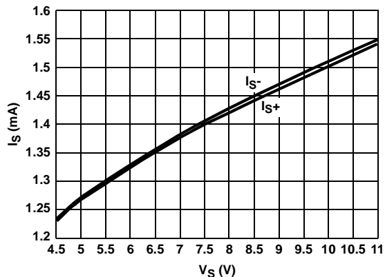
FIGURE 8. SUPPLY CURRENT vs SUPPLY VOLTAGE (PER AMPLIFIER)
