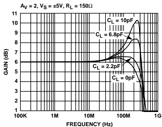
FIGURE 2. FREQUENCY RESPONSE FOR VARIOUS C L
