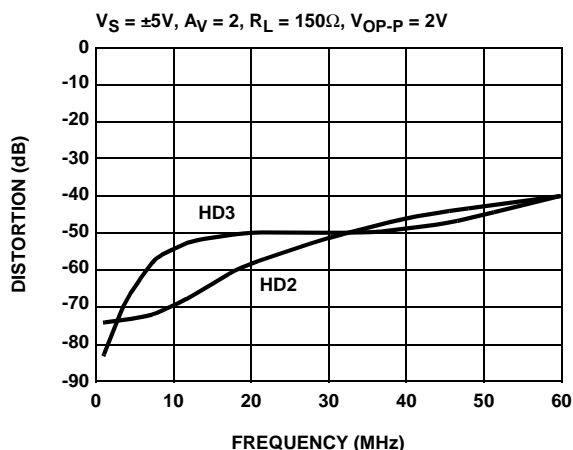
FIGURE 9. HARMONIC DISTORTION vs FREQUENCY
