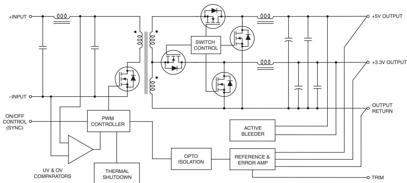
Figure 1. Simplified Schematic
