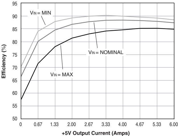
D24/D48 - 5 Volt Output Efficiency vs. Line and Load (+3.3V @ 700mA)
