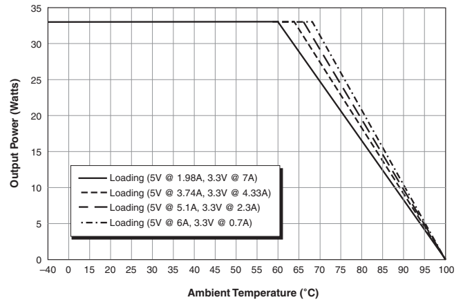
Output Power vs. Ambient Temperature V_{IN} = 24V , Natural Convection Air flow
