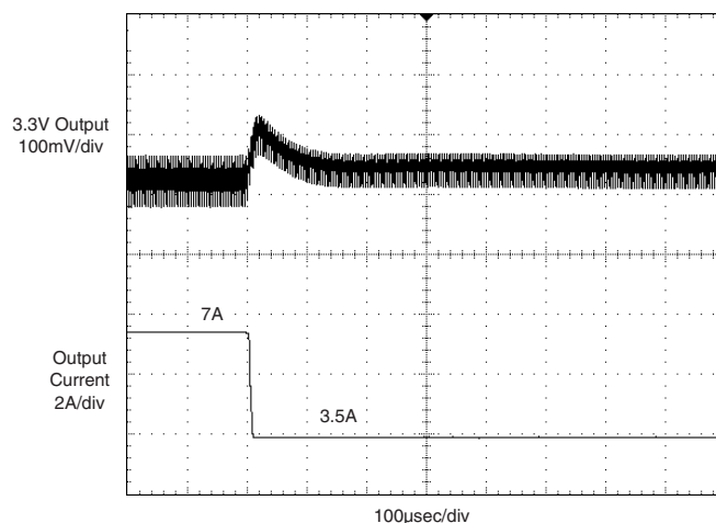
3.3V Output Full-Load to Half-Load Transient Response ( V_{IN} = nominal, 5V @ 600mA, external 1 \mu F output capacitors.)
