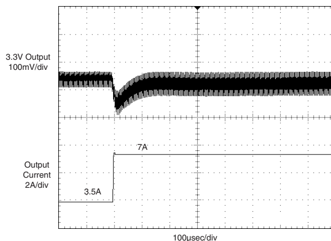
3.3V Output Half-Load to Full-Load Transient Response ( V_{IN} = nominal, 5V @ 600mA, external 1 \mu F output capacitors.)
