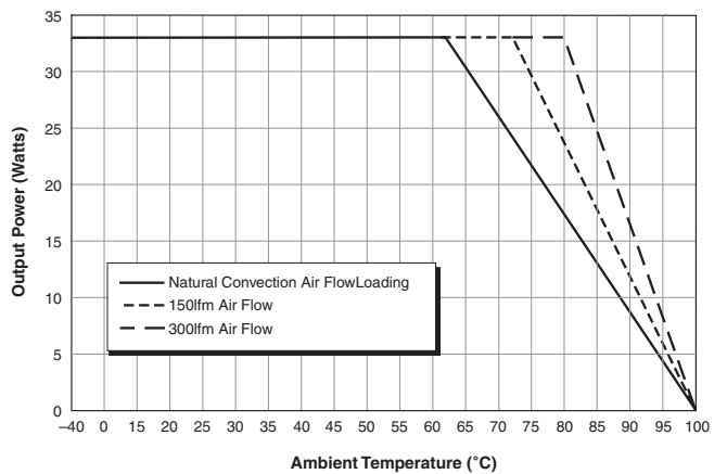
Output Power vs. Ambient Temperature V_{IN} = \text{Nominal} , 5V @ 3.74A/3.3V @ 4.33A
