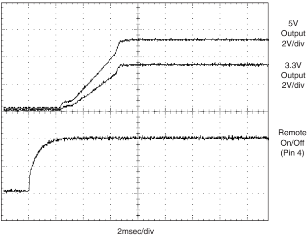
Start-Up from Remote On/Off Control (VIN = nominal, 5V @ 3A, 3.3V @ 4.5A, external 1μF output capacitors.)
