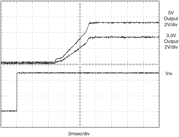
Start-Up from VIN (VIN = nominal, 5V @ 3A, 3.3V @ 4.5A, external 1μF output capacitors.)
