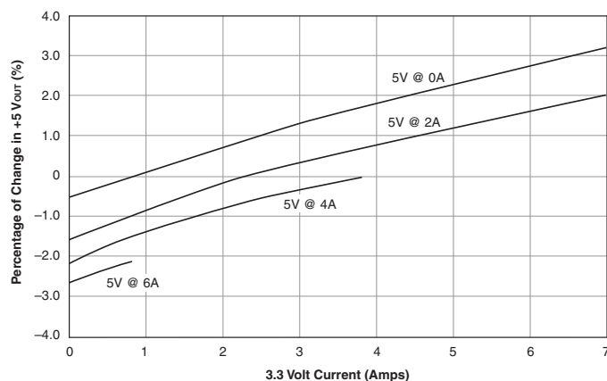
Cross Regulation Effects On +5V OUT (Reference Point 5V @ 4A, 3.3V @ 3.9A)
