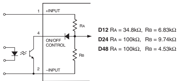
Figure 1. Internal Circuitry for No Suffix Models
