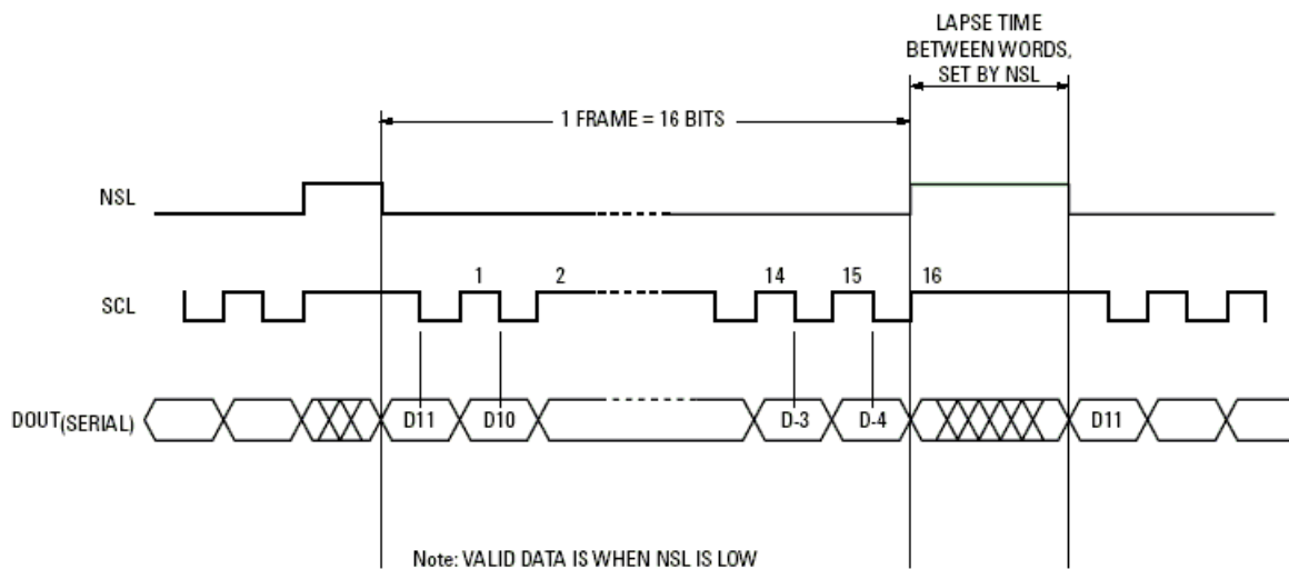
Figure 4. Timing Diagram
