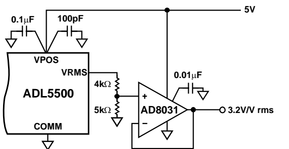
Figure 39. Output Buffering Options, Slope of 3.2 V/V rms at 900 MHz
