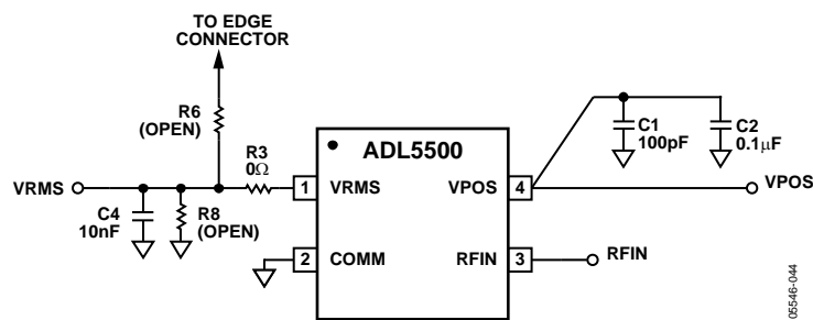
Figure 48. Evaluation Board Schematic
