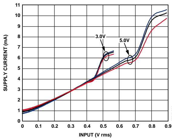
Figure 6. Supply Current vs. Input Level, Supplies 3.0 V and 5.0 V, Temperatures -40^\circ\text{C} , +25^\circ\text{C} , and +85^\circ\text{C}
