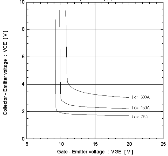
Collector-Emiiter voltage vs. Gate-Emiiter voltage Tj= 25°C (typ.)
