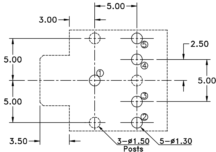
Recommended PCB Layout (Bottom View)
