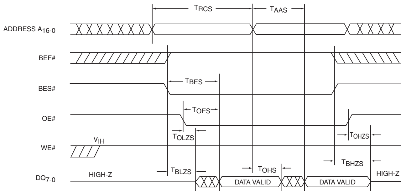
FIGURE 2: SRAM READ CYCLE TIMING DIAGRAM
