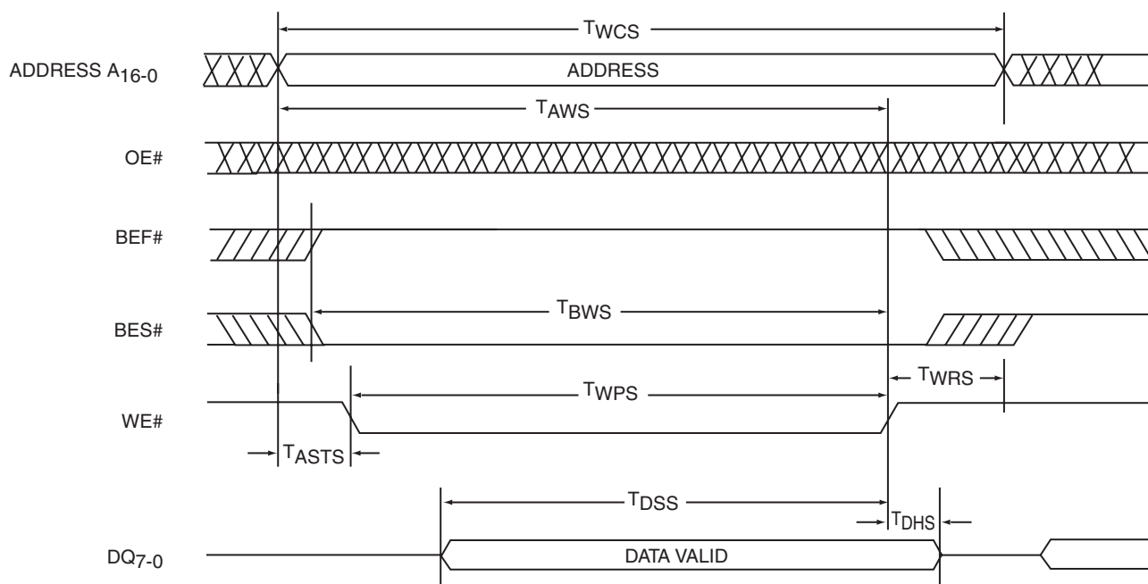
FIGURE 3: SRAM WRITE CYCLE TIMING DIAGRAM
