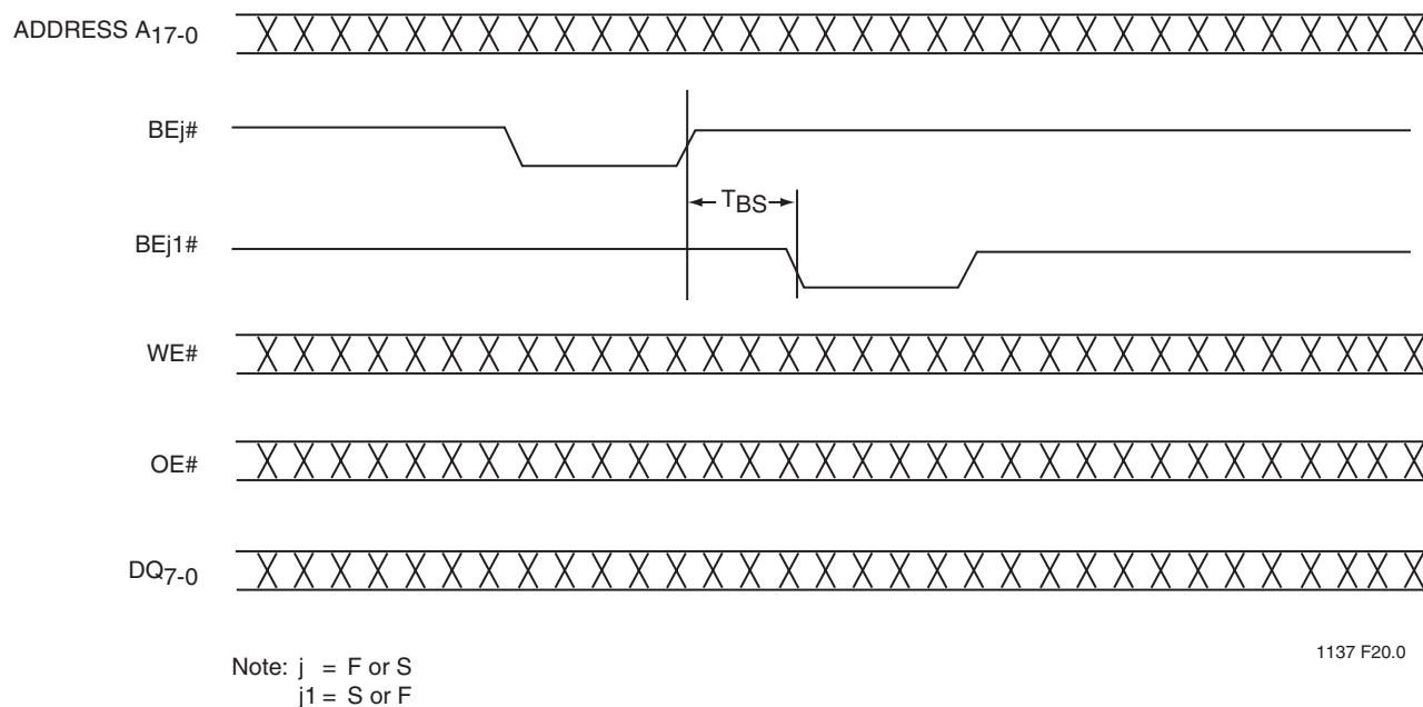
FIGURE 13: TIMING DIAGRAM FOR ALTERNATING BETWEEN FLASH/SRAM AND SRAM/FLASH
