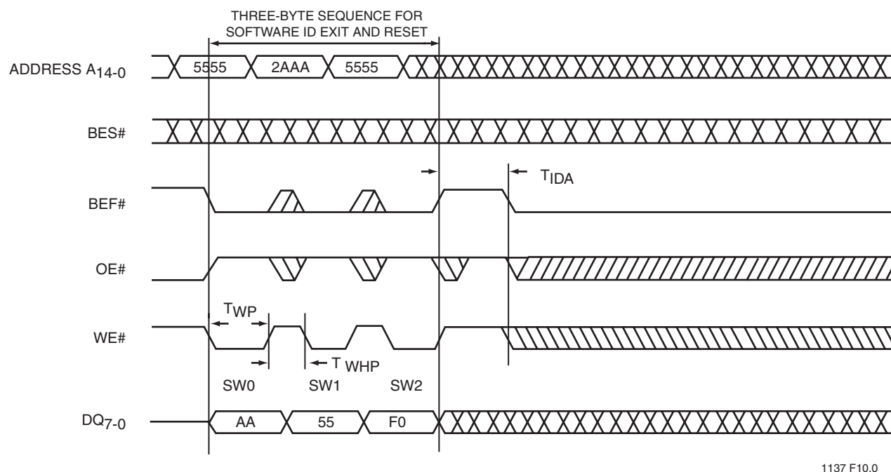
FIGURE 12: FLASH SOFTWARE ID EXIT AND RESET
