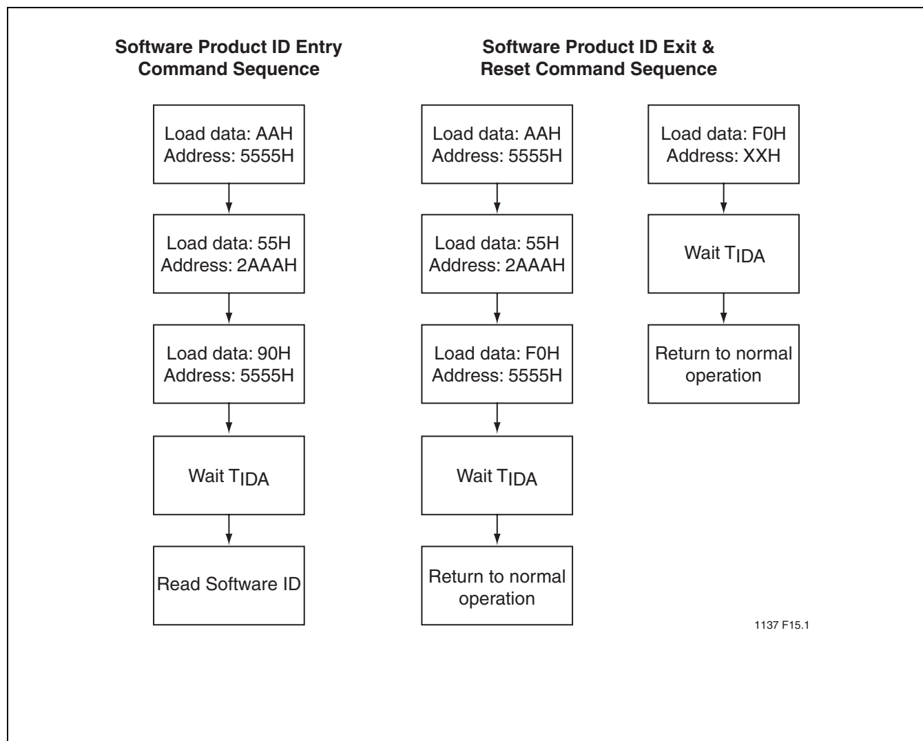
FIGURE 18: SOFTWARE PRODUCT COMMAND FLOWCHARTS
