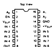
16-PIN HERMETIC DIP 16-PIN PLASTIC DIP
