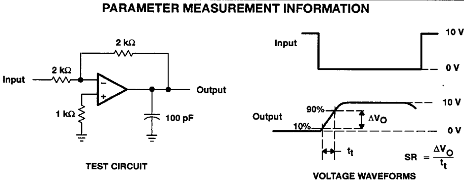
Figure 1. Slew Rate
