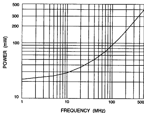
Fig. 8 Power Consumption
