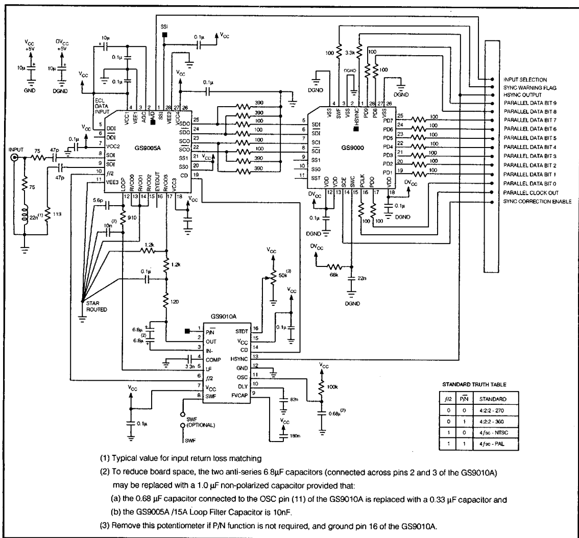
Fig. 10 Application Circuit - Adjustment Free Multistandard Serial to Parallel Converter
