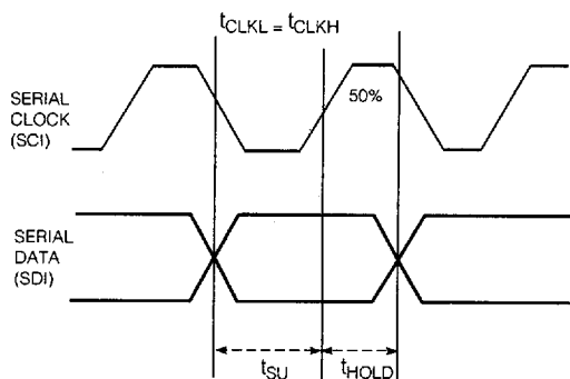
Fig. 7 Waveforms
