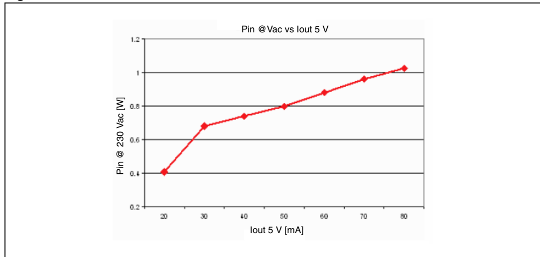
Figure 11. Pin at 230 Vac vs. Iout 5 V
