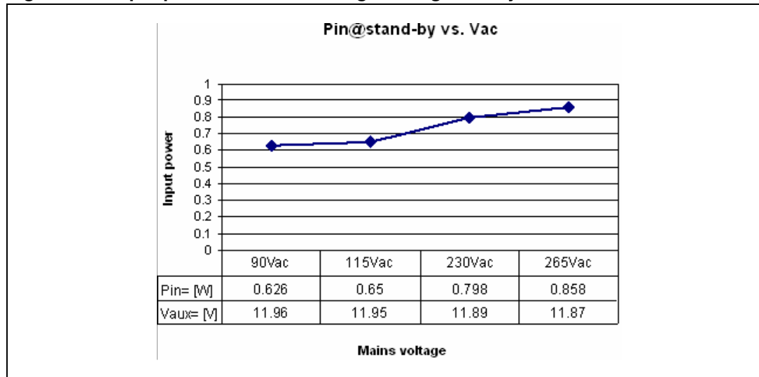
Figure 10. Input power vs. mains voltage during standby
