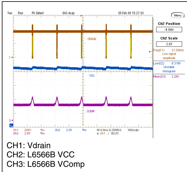
Figure 8. EVL6566B-40WSTB waveforms at 265 Vac - no load
