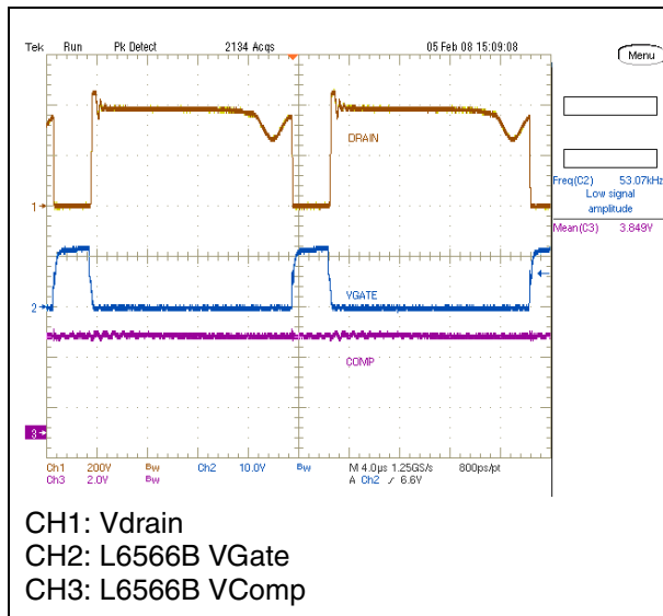
Figure 6. EVL6566B-40WSTB waveforms at 230 V - Pin=30 W
