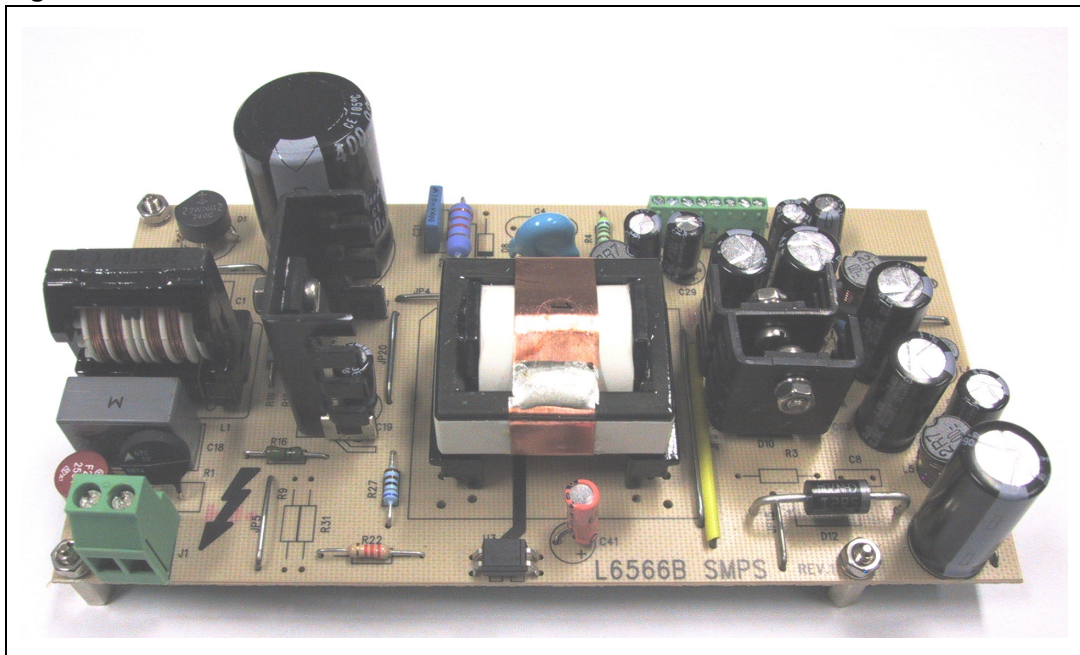
Figure 1. EVL6566B-40WSTB demonstration board
