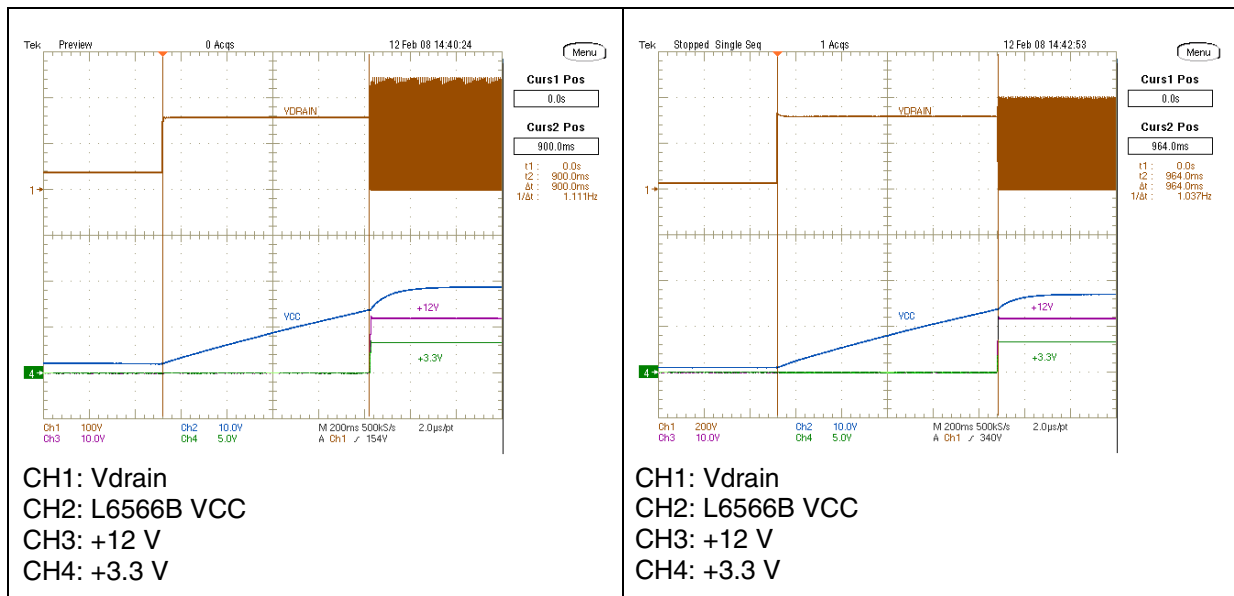
Figure 12. EVL6566B-40WSTB wakeup time at 115 Vac
