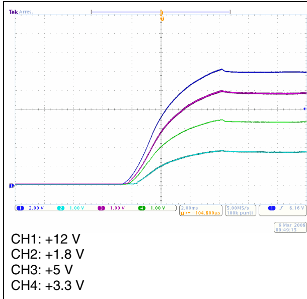
Figure 14. EVL6566B-40WSTB startup at 90 Vac - full load
