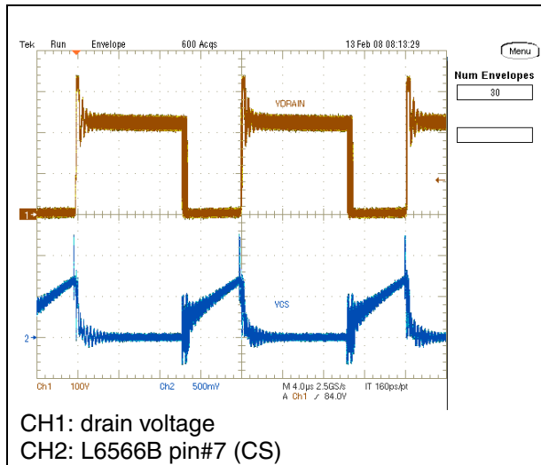
Figure 3. EVL6566B-40WSTB waveforms at 115 Vac-60 Hz - full load
