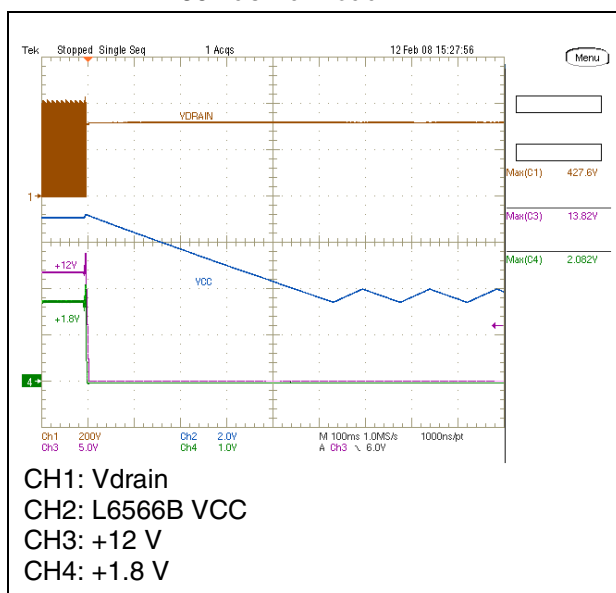
Figure 30. EVL6566B-40WSTB OVP at 230 Vac- full load
