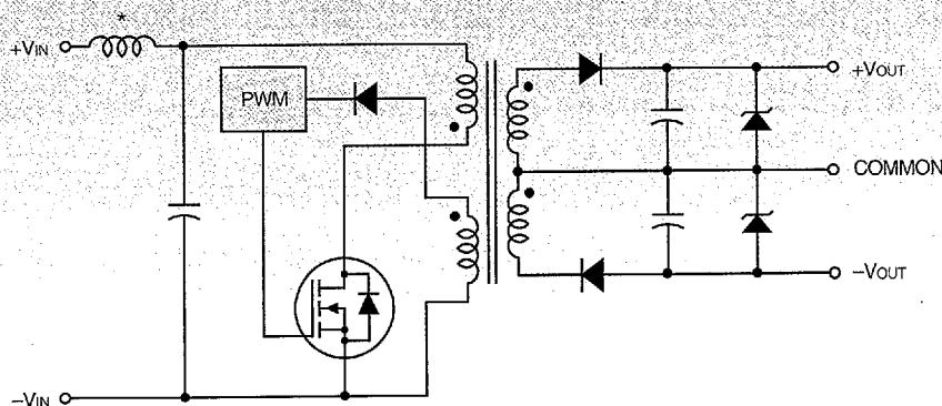
Figure 1. Simplified Schematic
