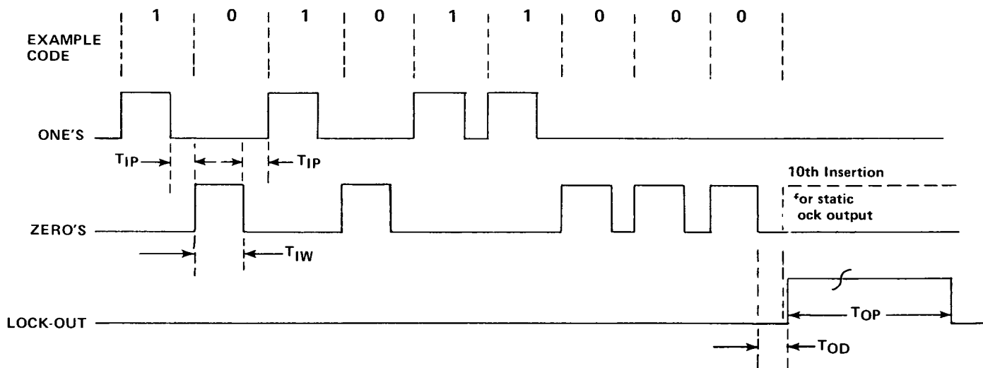
TIMING DIAGRAM Figure 2
