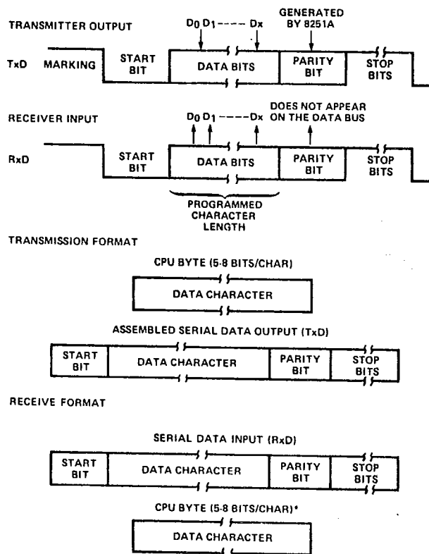
Figure 9. Asynchronous Mode
