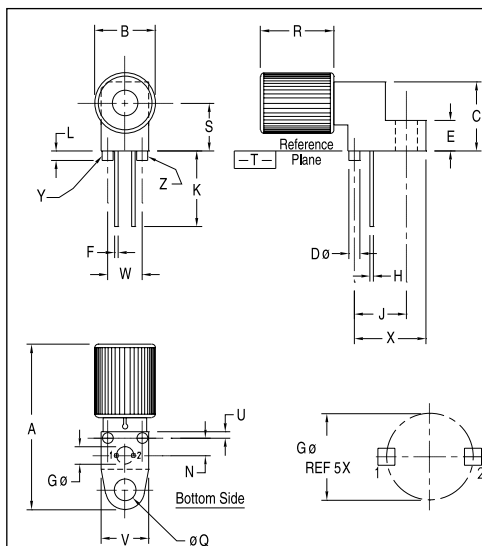
FIGURE 4. Case outline.
