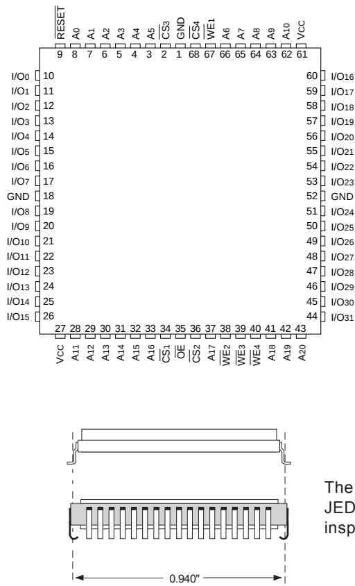
FIG. 2 PIN CONFIGURATION FOR WF2M32-XG2UX5
