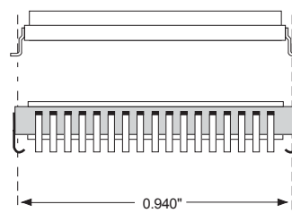
FIG. 11 ALTERNATE PIN CONFIGURATION FOR WF2M32U-XG2UX5
