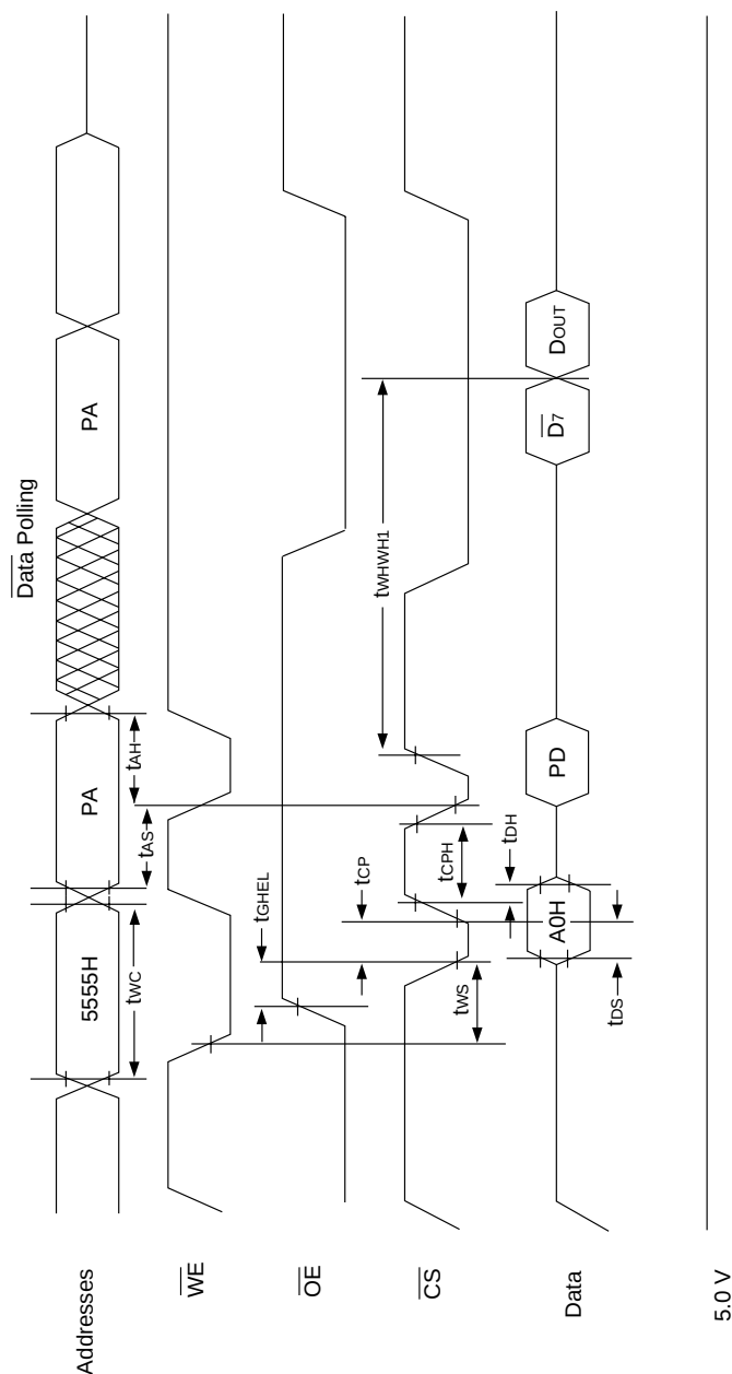
ALTERNATE \overline{\text{CS}} CONTROLLED PROGRAMMING OPERATION TIMINGS
