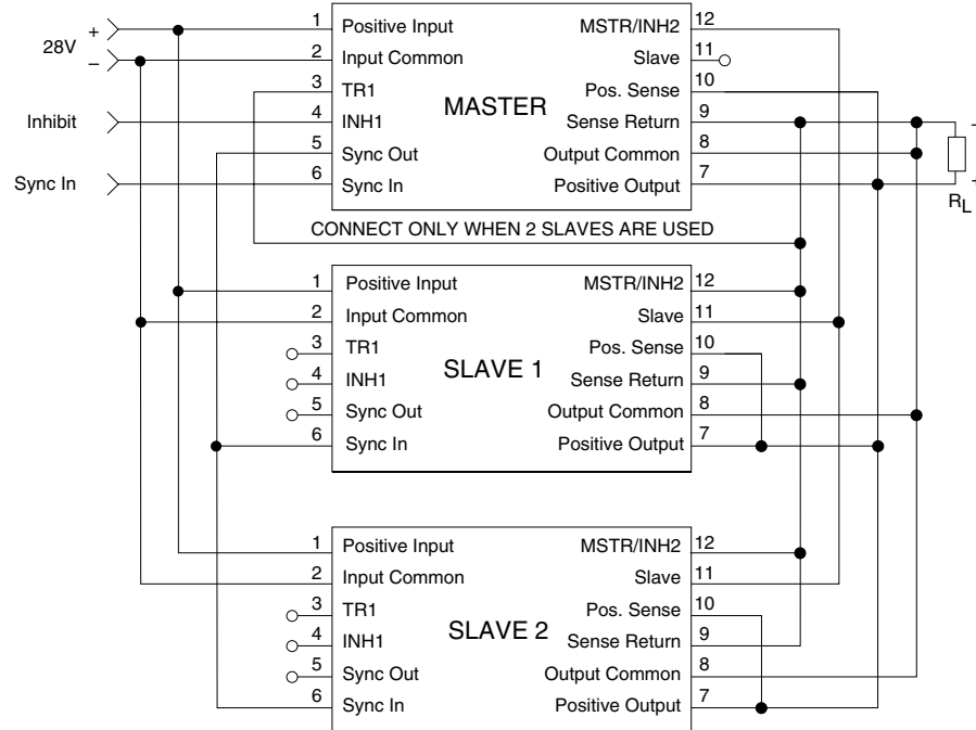
FIGURE 2: PARALLEL CONNECTIONS
