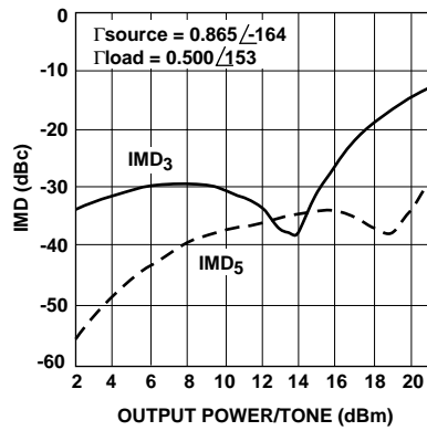
Figure 5. IMD_3 , IMD_5 vs. Output Power (per tone) at V_{CE} = 3.0\text{ V} and I_{CQ} = 15\text{ mA} , Frequency = 900\text{ MHz} .
