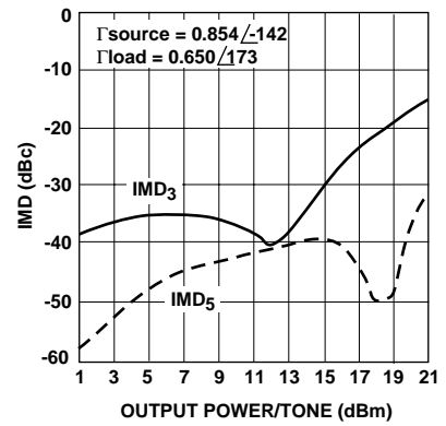
Figure 6. IMD_3 , IMD_5 vs. Output Power (per tone) at V_{CE} = 3.0\text{ V} and I_{CQ} = 15\text{ mA} , Frequency = 1900\text{ MHz} .
