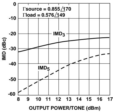
Figure 4. IMD_3 , IMD_5 vs. Output Power (per tone) at V_{CE} = 3.0\text{ V} and I_{CQ} = 15\text{ mA} , Frequency = 450\text{ MHz} .
