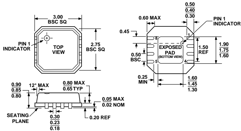
Figure 71. 8-Lead Lead Frame Chip Scale Package [LFCS] 3 mm x 3 mm Body (CP-8-2)—Dimensions shown in millimeters
