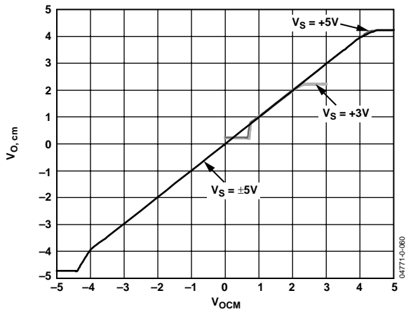
Figure 55. V_{O,cm} vs. V_{OCM} Input Voltage
