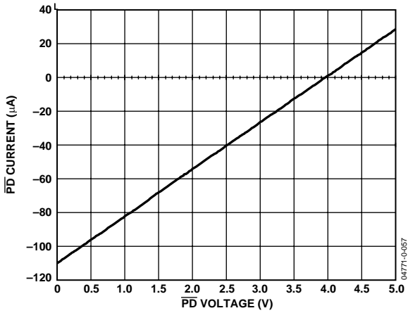
Figure 56. \overline{PD} Current vs. \overline{PD} Voltage
