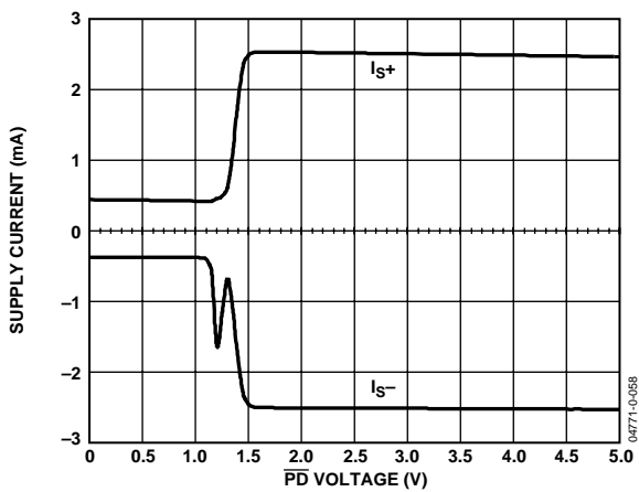
Figure 57. Supply Current vs. \overline{PD} Voltage
