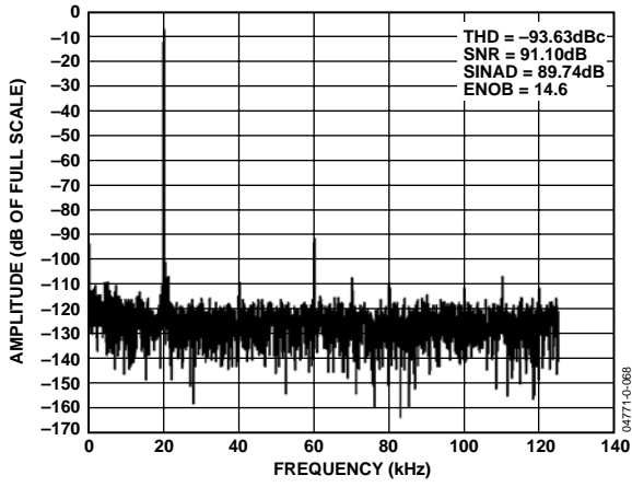
Figure 68. AD8137 Performance on Single 5 V Supply, -1.82 dBFS
