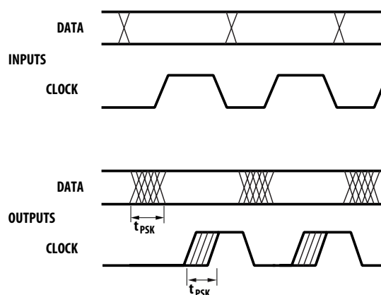
Figure 11. Parallel data transmission example.
