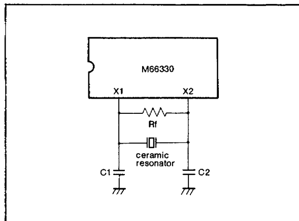
Fig. 17 Clock generator
