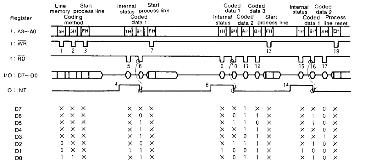
Fig. 5 Output sequence for one line of MH-coded data (MPU bus)
