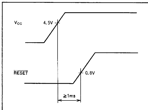
Fig. 16 Requirements for power on reset
