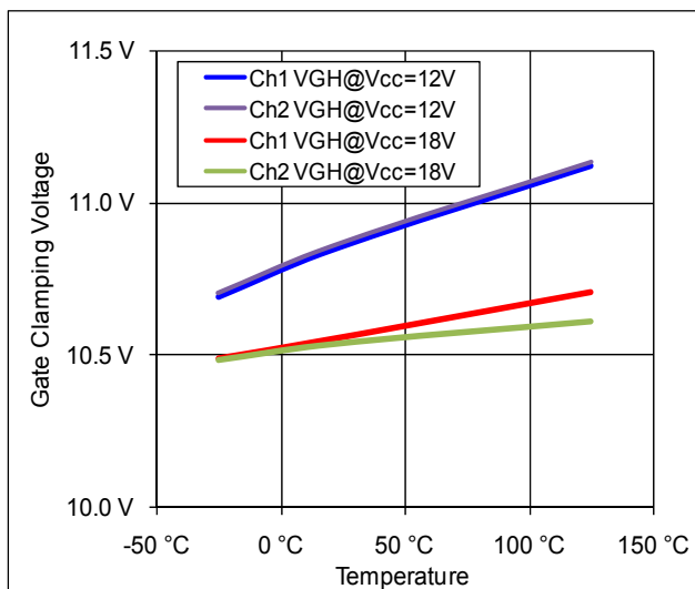
Figure 17: Gate Clamping Voltage vs. Temperature
