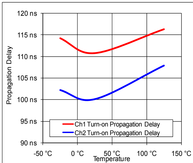
Figure 15: Turn-on Propagation Delay vs. Temperature
