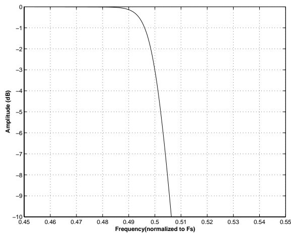
Figure 21. Single-Speed (fast) Transition Band (detail)
