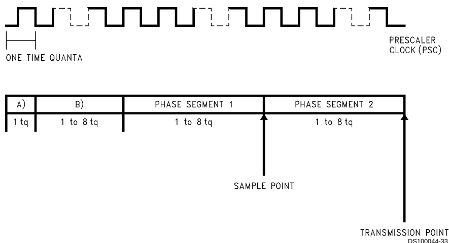
FIGURE 28. Bit Timing
