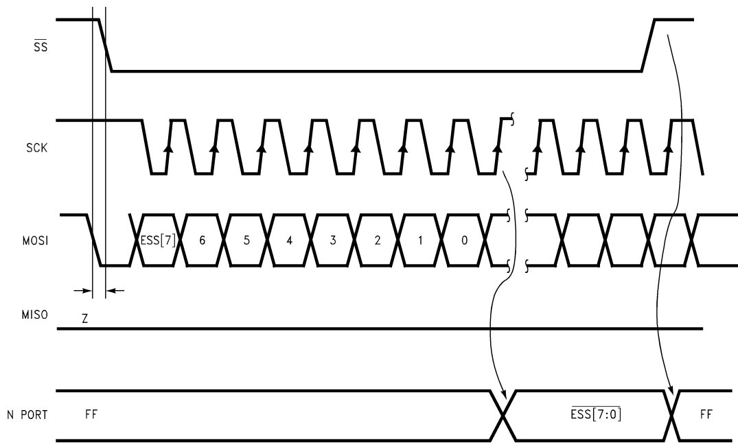
FIGURE 39. Programming the SPI Expander
