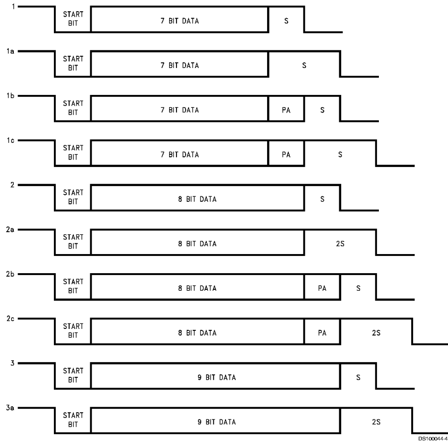
FIGURE 45. Framing Formats
