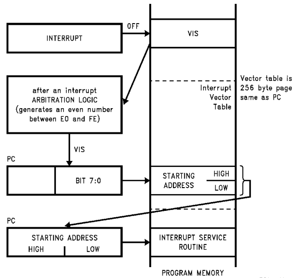
FIGURE 32. VIS Operation
