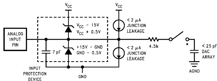
FIGURE 43. A/D Pin Model (Single Ended Mode)
