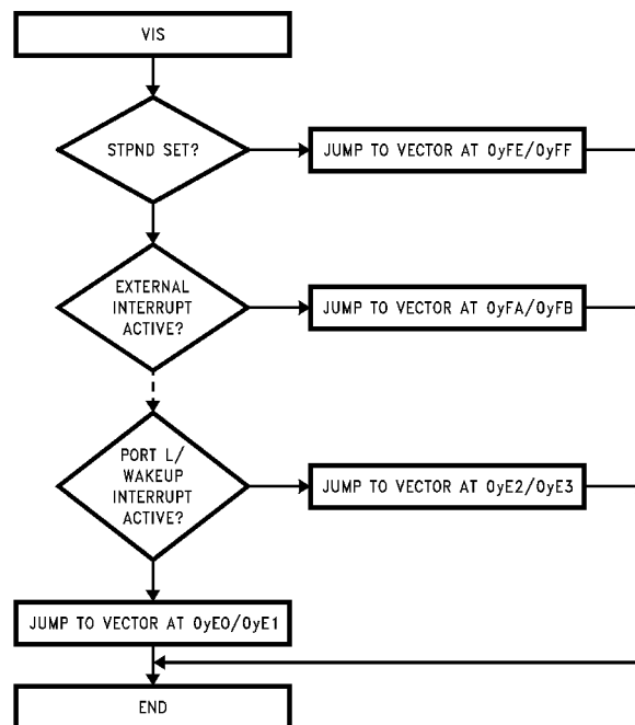
FIGURE 33. VIS Flowchart
