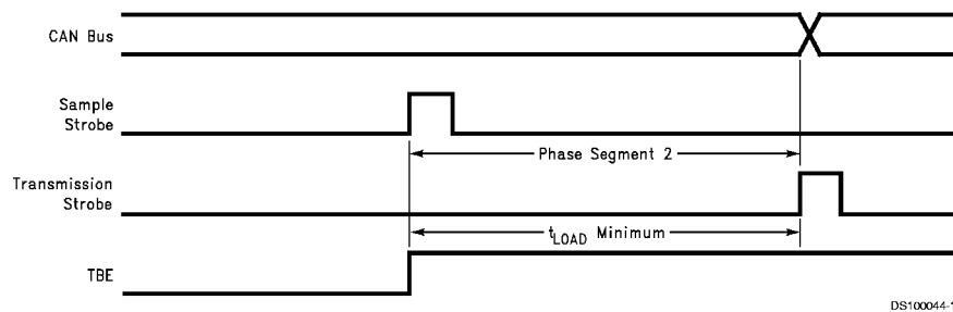
FIGURE 16. TBE Timing
