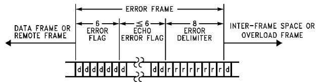
FIGURE 19. CAN Data Transmission Frames
