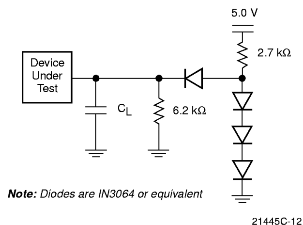
Figure 7. Test Setup
