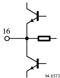
Figure 14. Video demodulator output (Pin 16)
