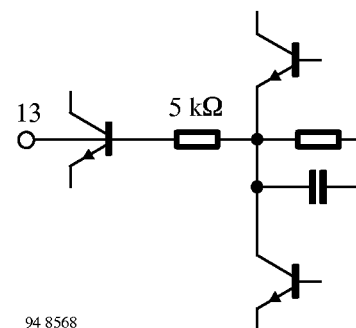
Figure 11. De-emphasis (Pin 13)
