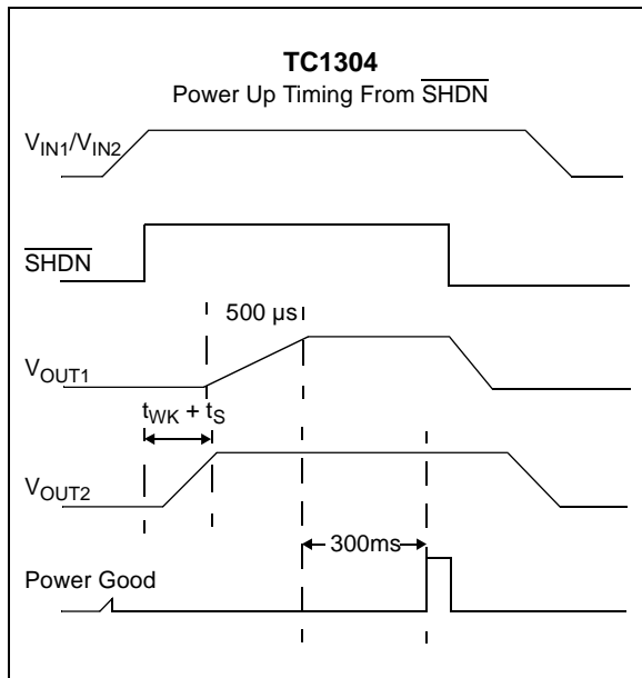
FIGURE 4-3: TC1304 Power-up Timing from \overline{\text{SHDN}} .
