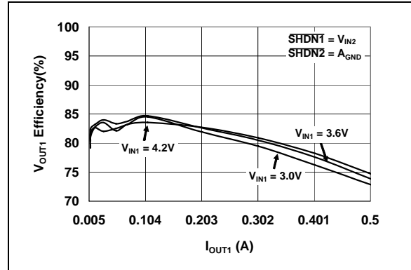
FIGURE 2-6: V_{OUT1} Output Efficiency vs. I_{OUT1} ( V_{OUT1} = 1.2\text{V} ).
