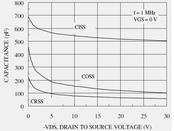
Figure 4. Capacitance Characteristics
