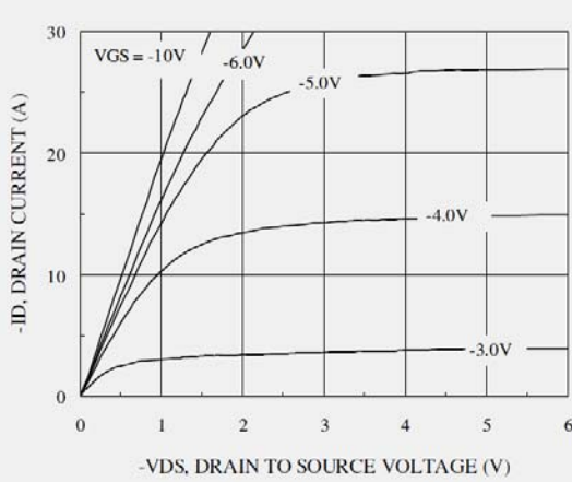
Figure 1. On-Region Characteristics
