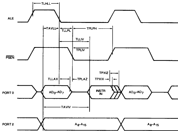
External Program Memory Read Cycle
