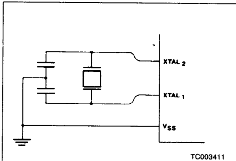
Figure 1. Crystal Oscillator
