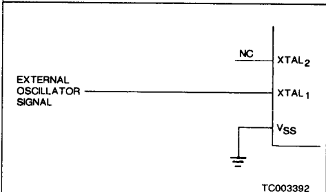
Figure 2. External Drive Configuration
