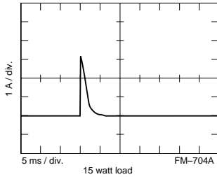
Inrush Current
