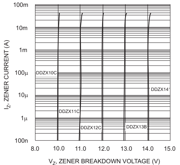
Fig. 5 Typical Reverse Characteristics, DDZX10C - DDZX14
