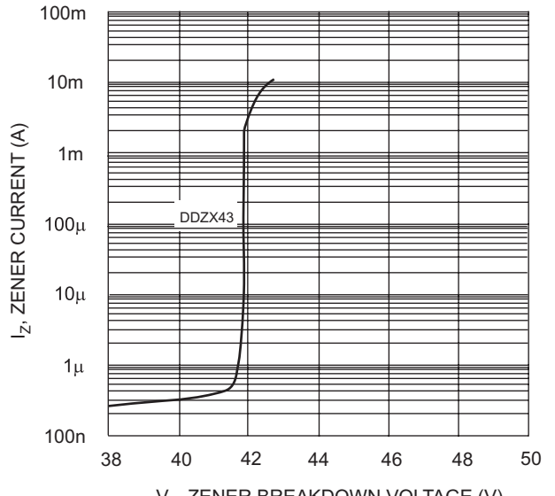
Fig. 9 Typical Reverse Characteristics, DDZX43
