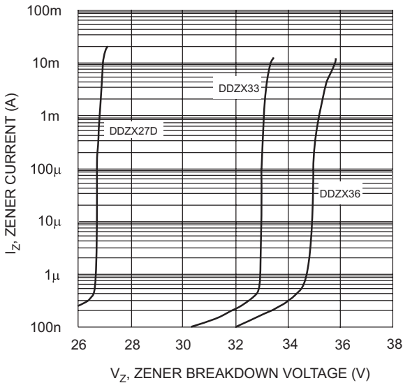
Fig. 8 Typical Reverse Characteristics, DDZX27D - DDZX36
