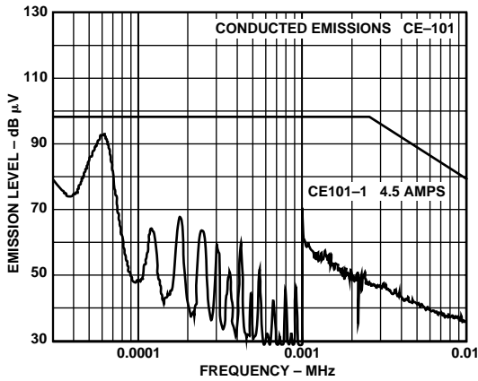
Figure 13. Conducted Emissions, MIL-STD-461D, CE101, +28 V Hot Line 100 W Load
